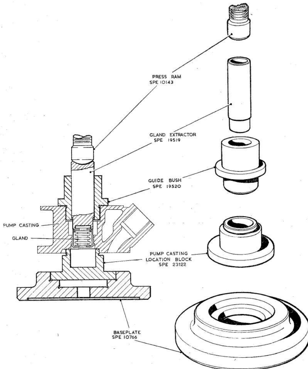
Fig. 3. Removing the bellows gland
