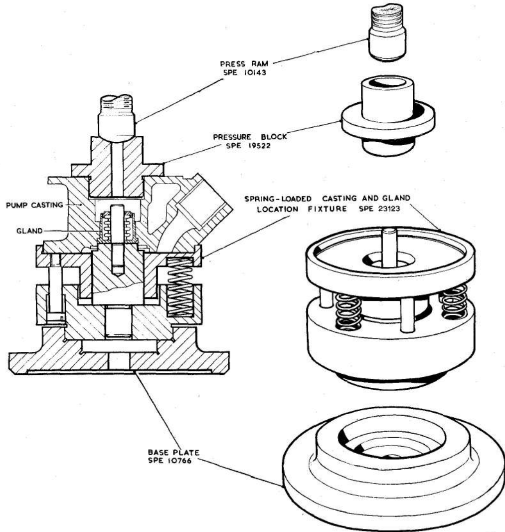
Fig. 4. Assembling the bellows gland
