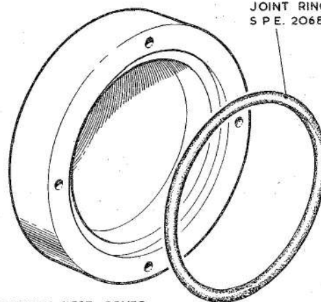
D PRESSURE TEST COVER S P E. 17628
