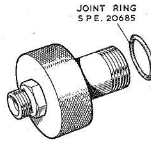
B PRESSURE TEST ADAPTOR. S P E. 20679
