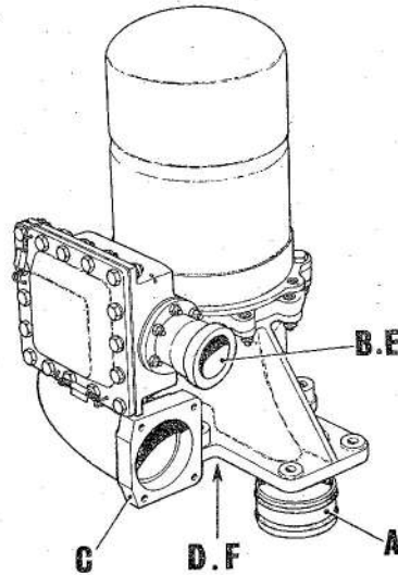
A PRESSURE TEST FIXTURE. S P E. 17397
