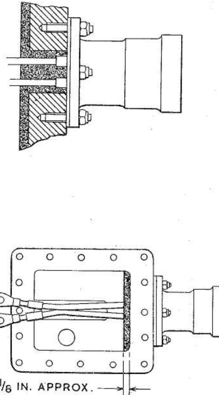
Fig. 10. Electrical connection sealing: instruction diagram
