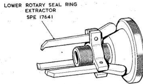
Fig 5. Tool for withdrawing the lower rotary seal ring
