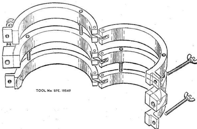
Fig. 1. Tool for removing top and pump casings
