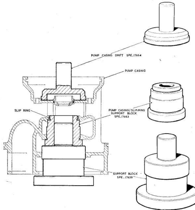
Fig. 30. Tools for assembling the upper impeller slip-ring into the pump casing
