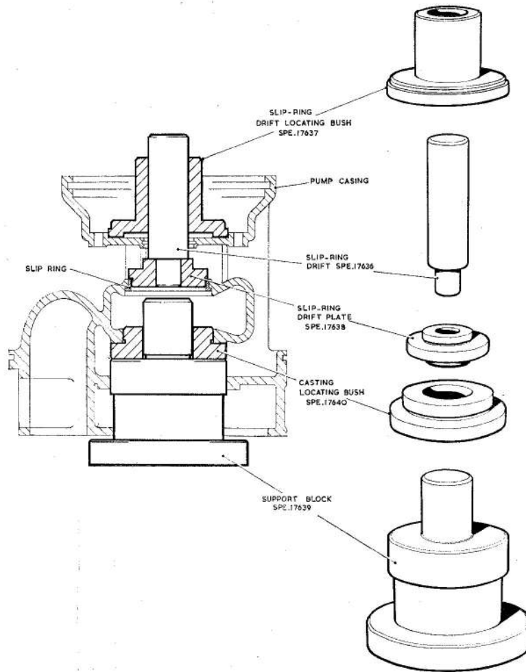
Fig. 13. Tools for removing the upper impeller slip-ring from the pump casing
