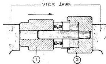
ASSEMBLY OF SLEEVED UPPER BEARING
