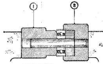
REMOVAL OF BEARING FROM SLEEVE
