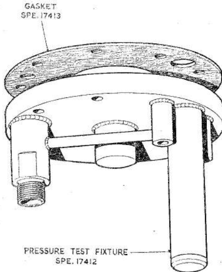
Fig. 14. Tools for pressure testing the pump assembly
