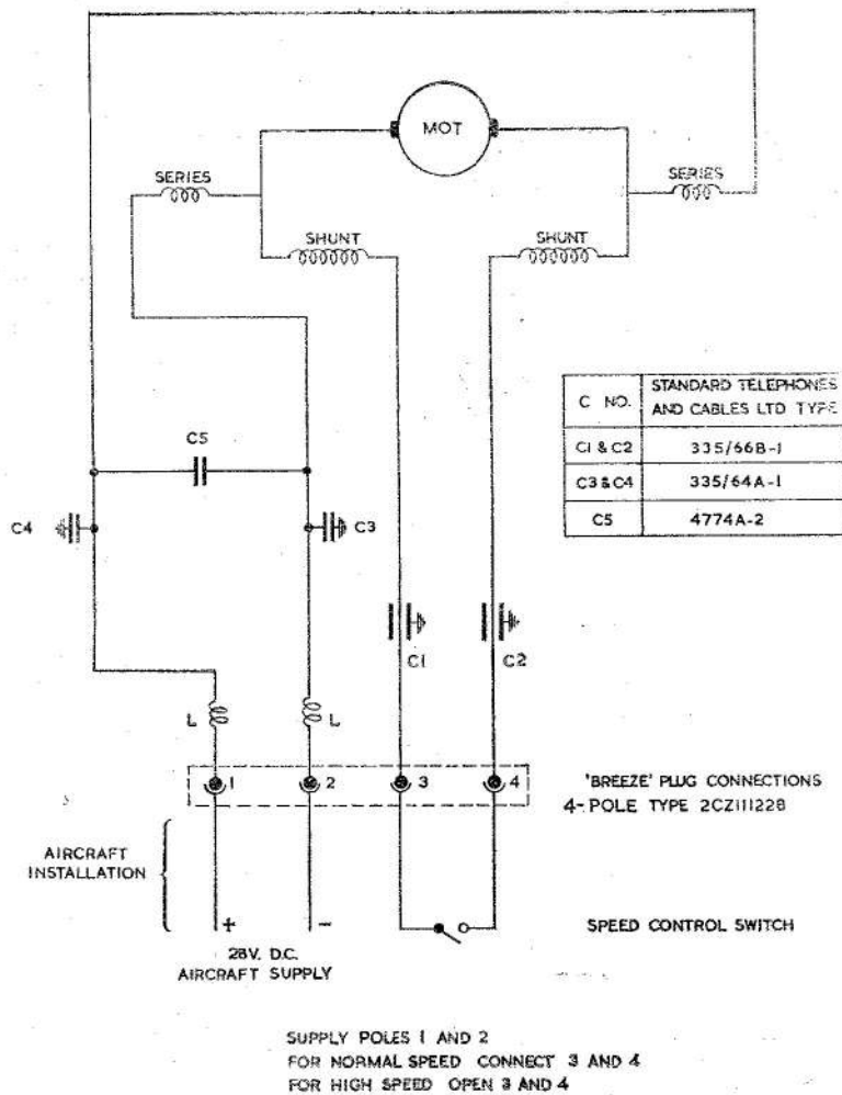
Fig. 3. Circuit diagram: SPE.2009A series fuel pumps
