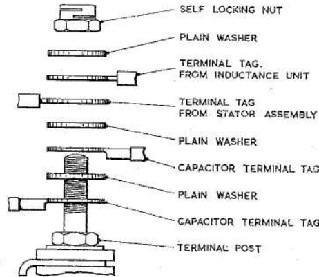
Fig. 9. Exploded view of terminal assembly (suppression unit)
