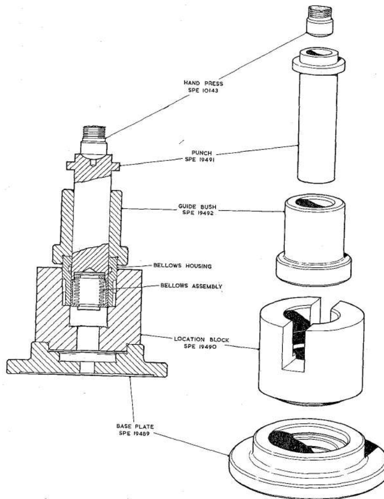
Fig. 19. Bellows gland removal from housing
