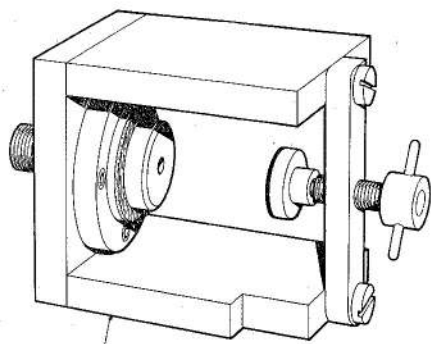
GLAND HOUSING SUB-ASSEMBLY PRESSURE TEST FIXTURE SPE. 19518
