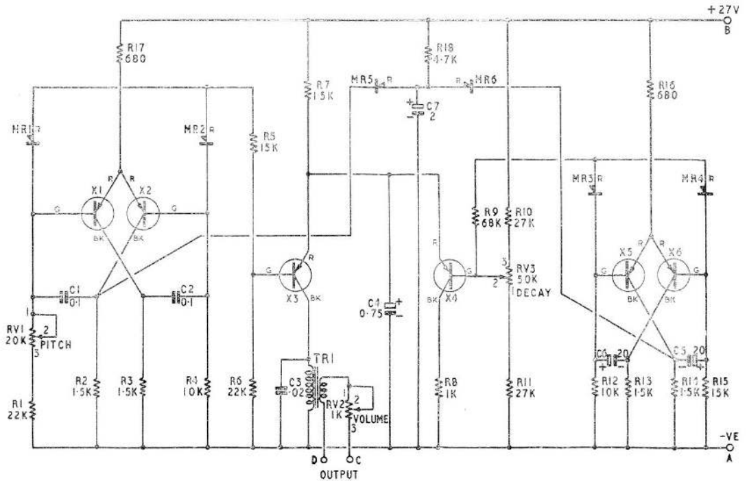
Fig. 3. Circuit diagram
