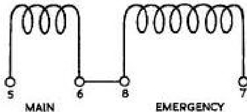
Fig. 3. Diagram of internal connections
