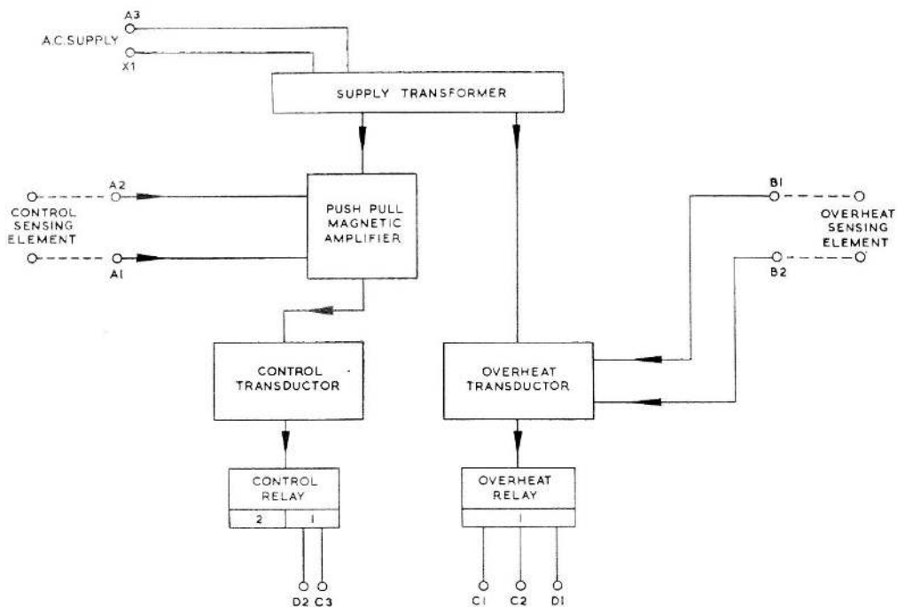
Fig. 3. Block diagram
