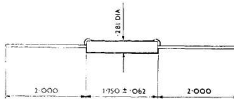
Fig 1. Resistor, Rotax, Type N79776
