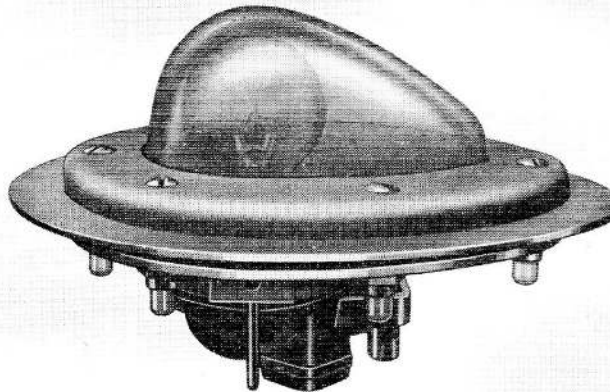
Fig. 1. Fuselage navigation lamp, Type FNL/50
