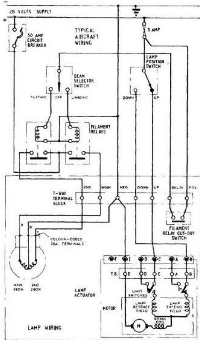
Fig. 2. Circuit diagram
