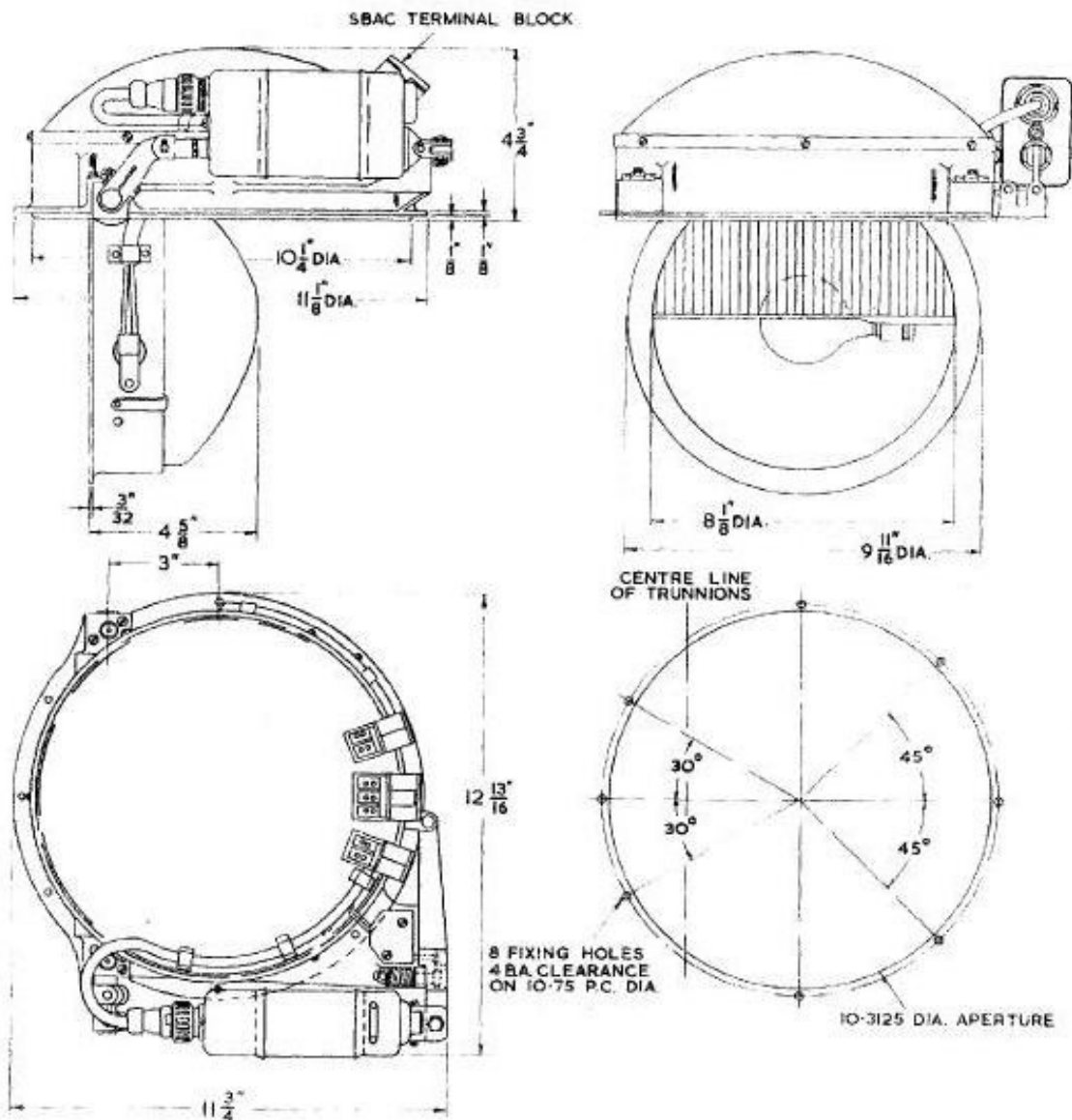
Fig. 3. Installation drawing
