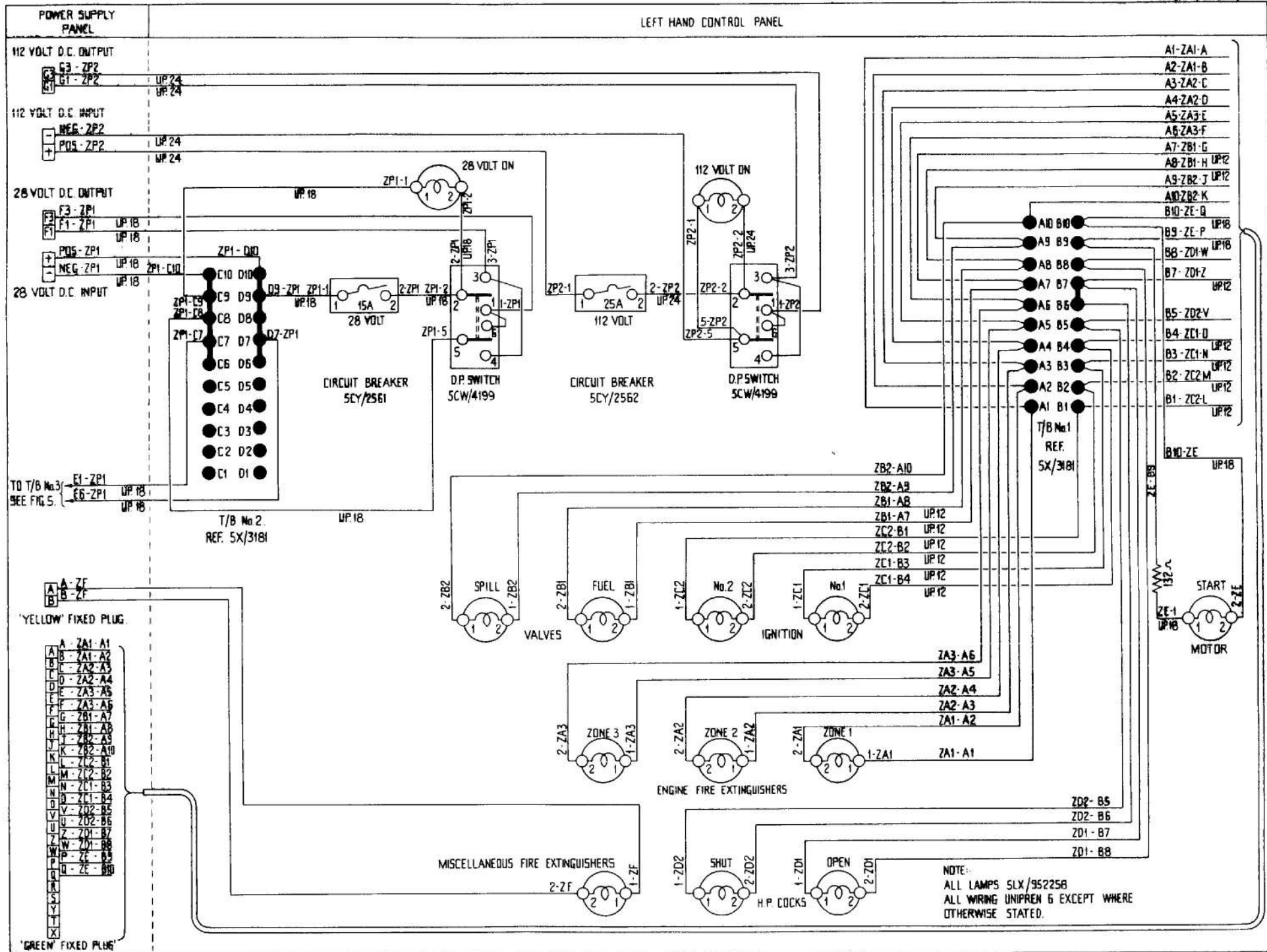
Fig.4. Left hand control panel wiring diagram
