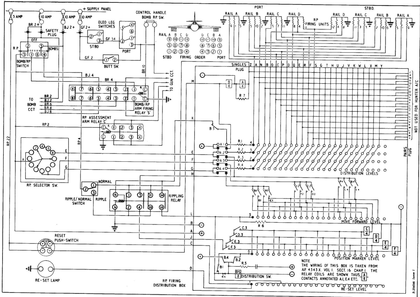
Fig. 8 R.P. (Theoretical)
