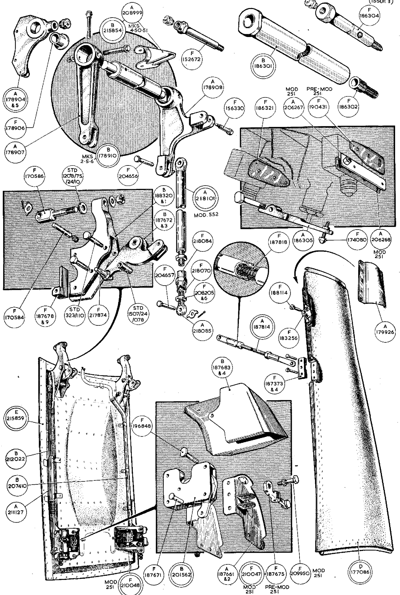
NOSE UNDERCARRIAGE
