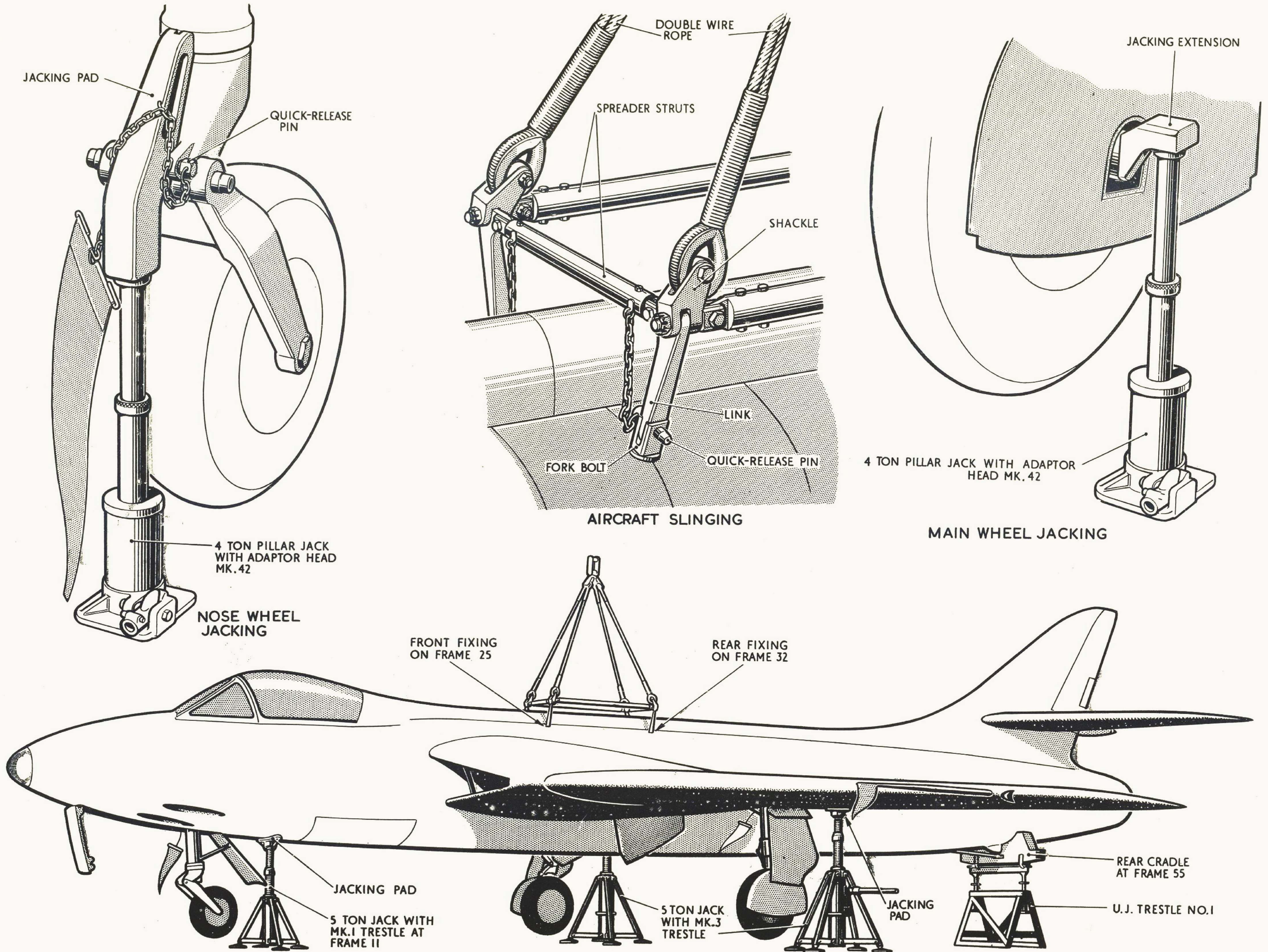
FIG. 4 JACKING, TRESTLING AND SLINGING
