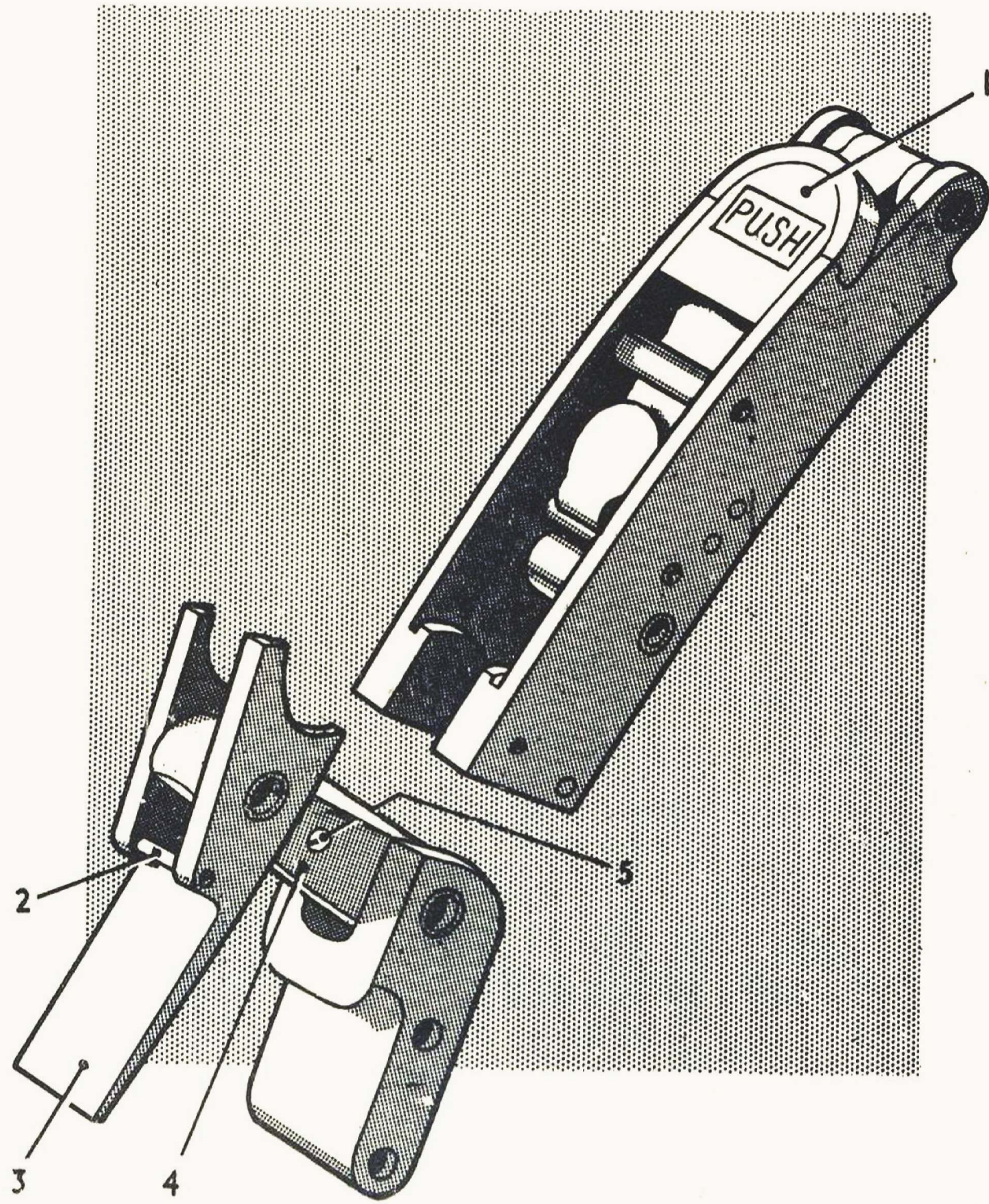
FIG. 3 TOGGLE FASTENER
