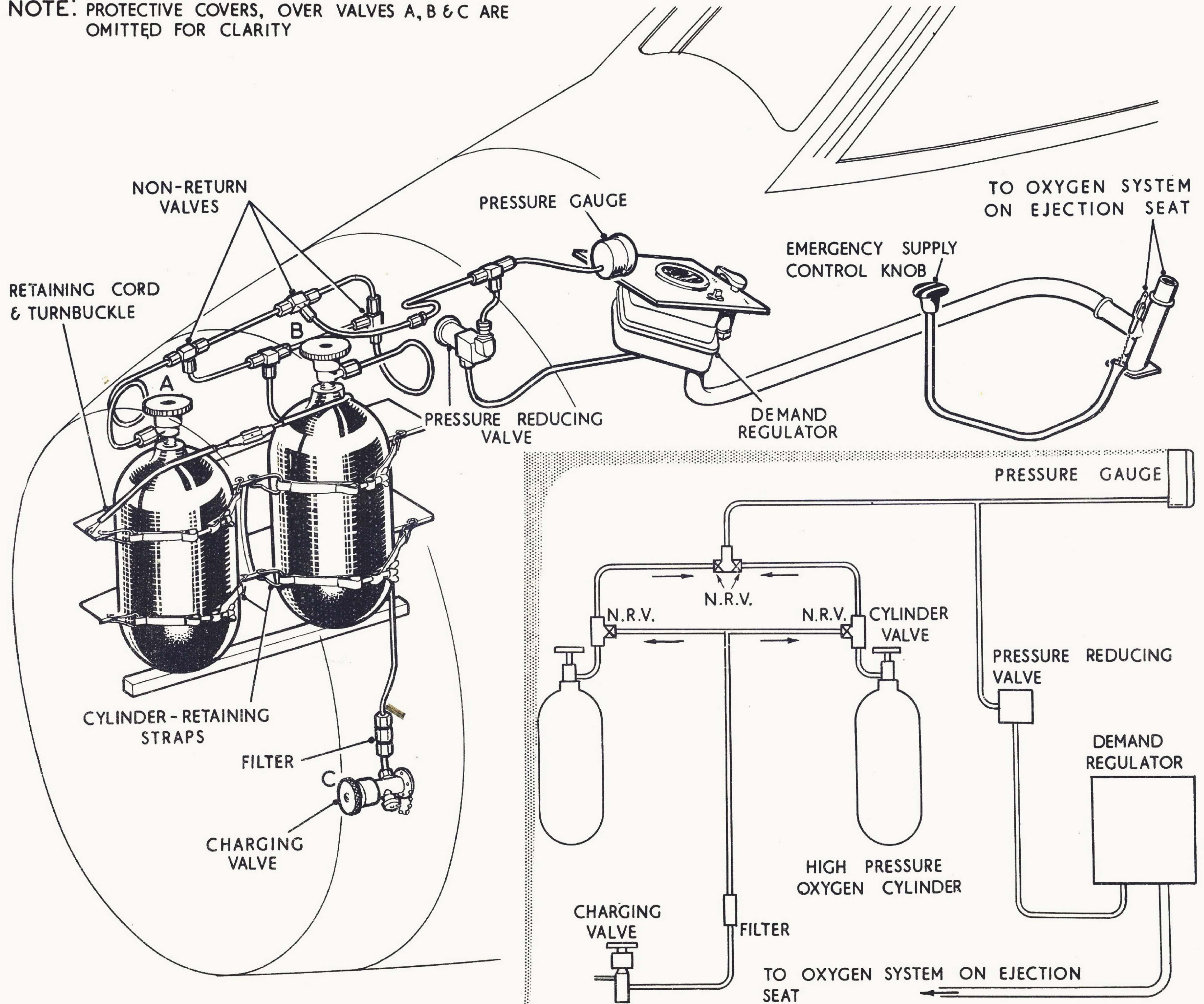
FIG. 1 OXYGEN INSTALLATION AND DIAGRAM
