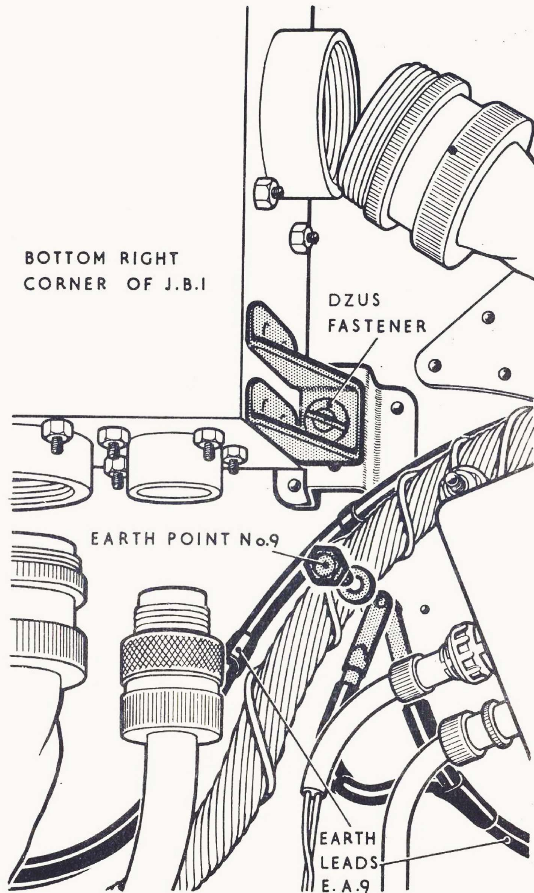
FIG.1 J.B.I LOWER ATTACHMENTS AND EARTH POINT No.9
