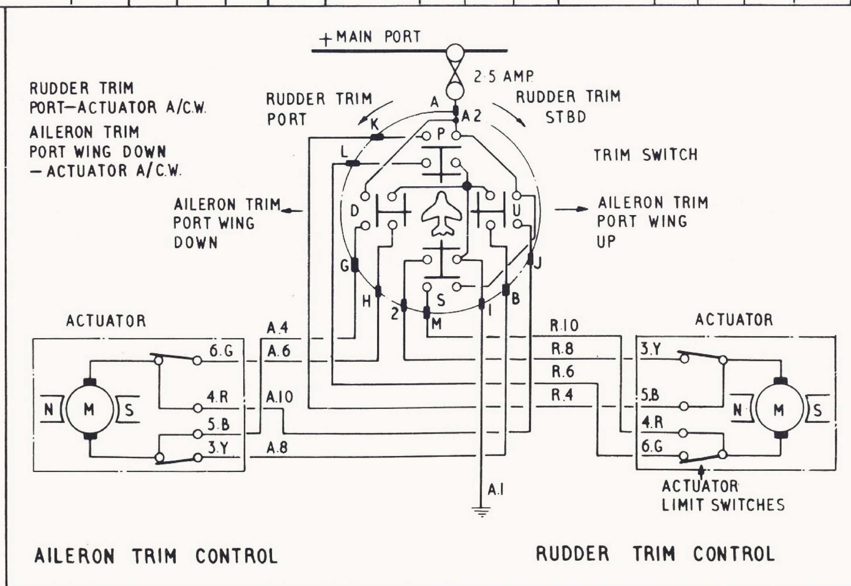
FIG. 1. RUDDER AND AILERON TRIM CONTROLS AND INDICATORS
