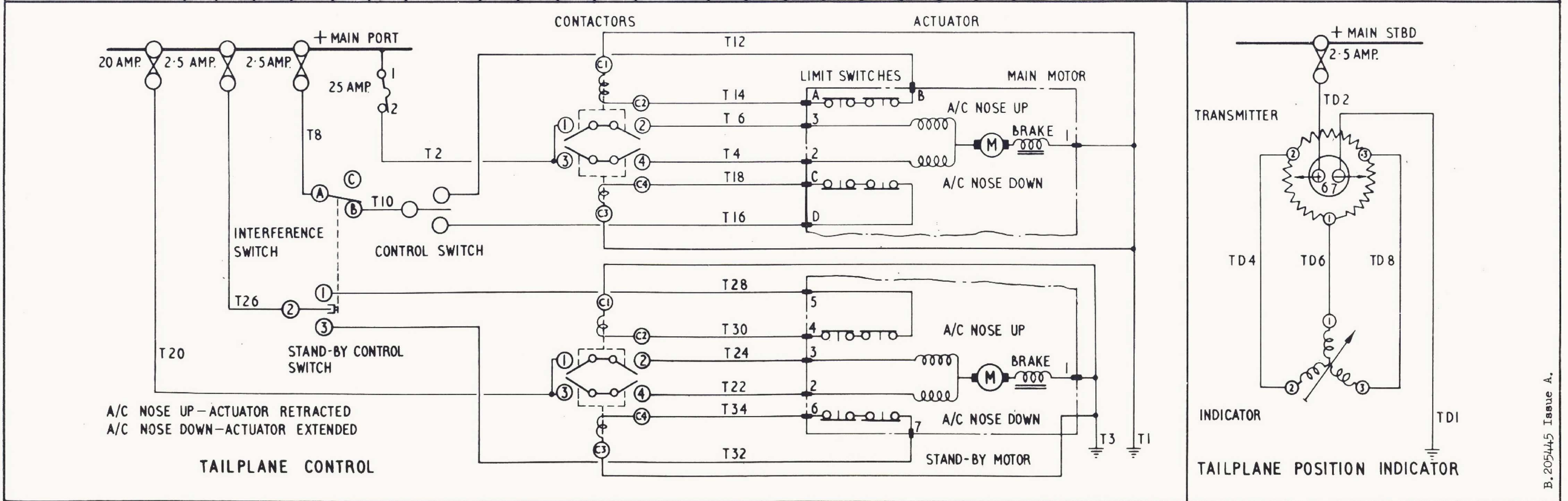
FIG. 1. TAIL PLANE CONTROL AND POSITION INDICATOR
