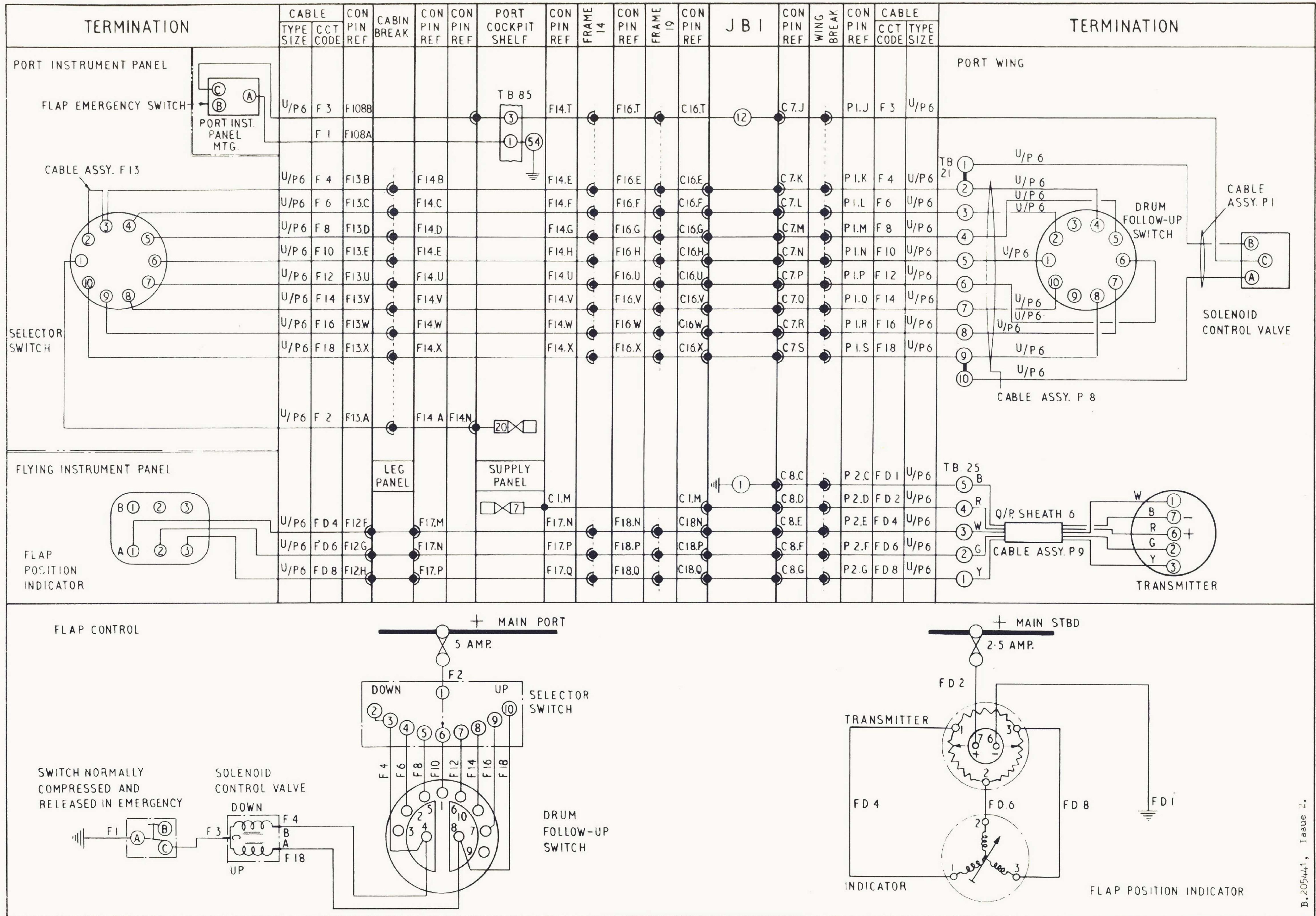
FIG. 1. FLAP CONTROL AND POSITION INDICATOR
