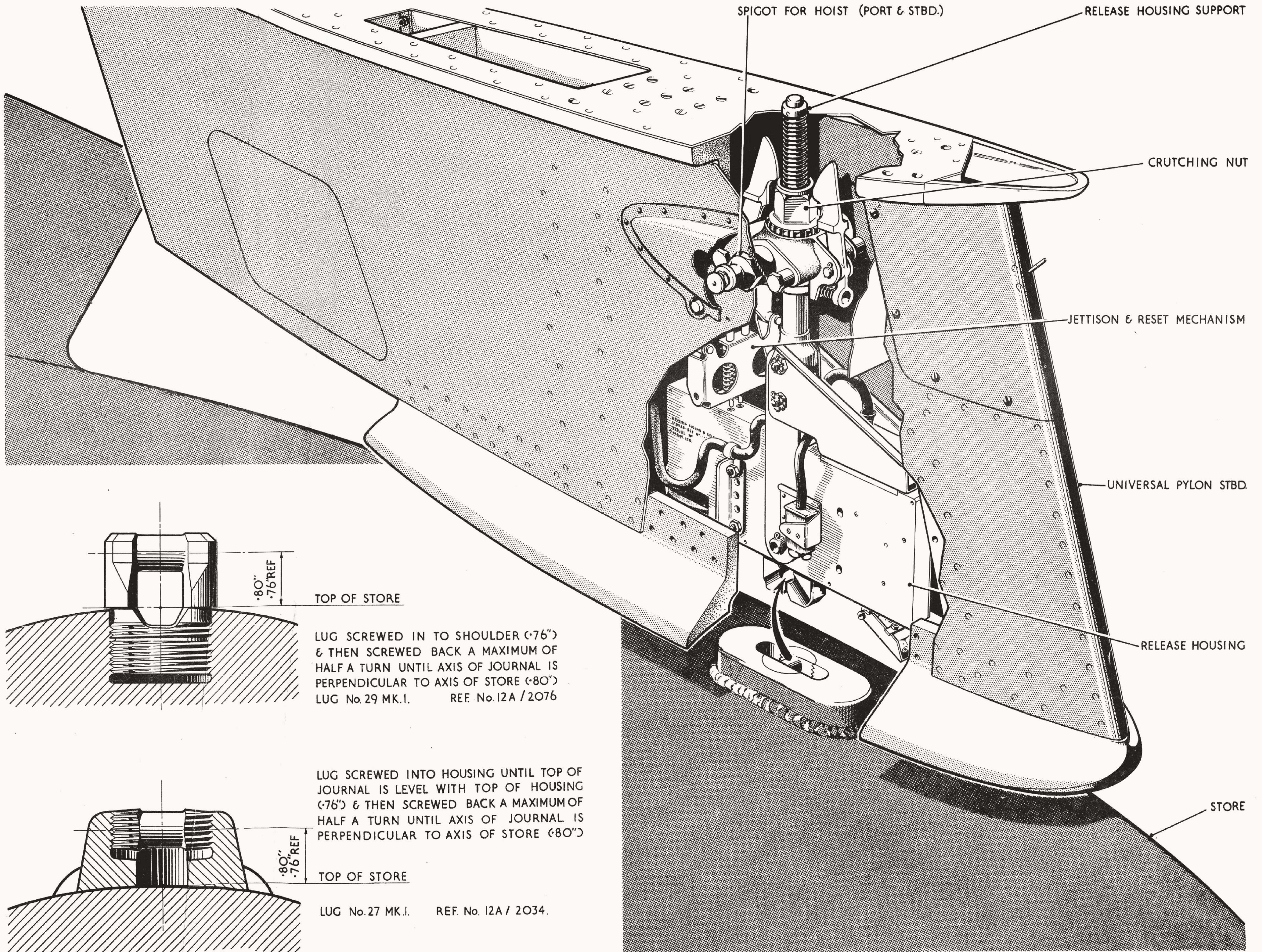
FIG. I BOMB INSTALLATION
