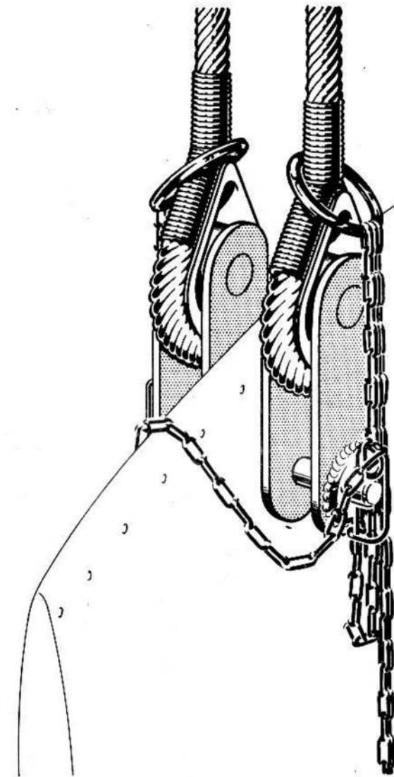
FIG. 4. ATTACHMENT OF RUDDER SLING
