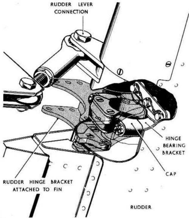
FIG. 3. RUDDER OPERATING LEVER AND BOTTOM HINGE
