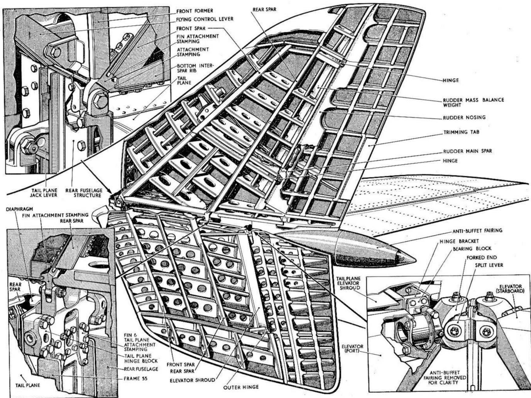
FIG. 1 TAIL UNIT
