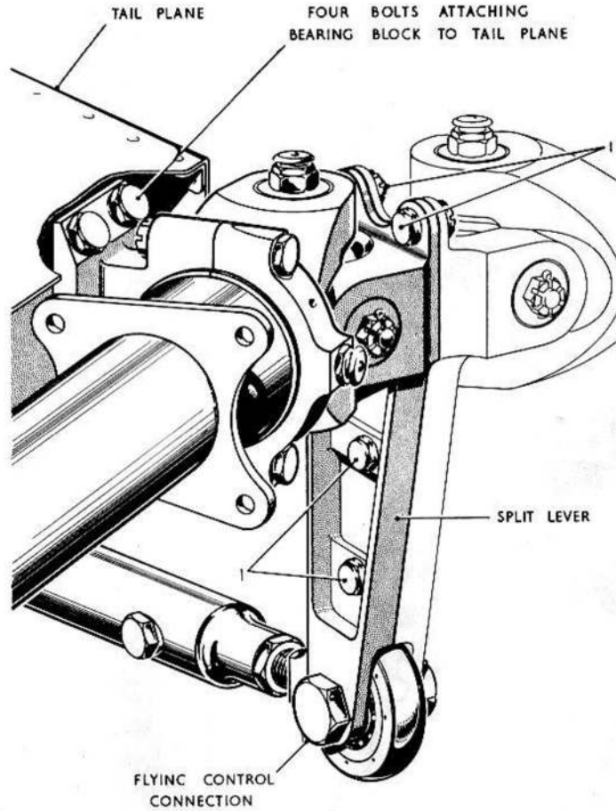
FIG. 9. SPLIT LEVER CONNECTING PORT & STAR'BD ELEVATORS & INNER HINGE BEARING
