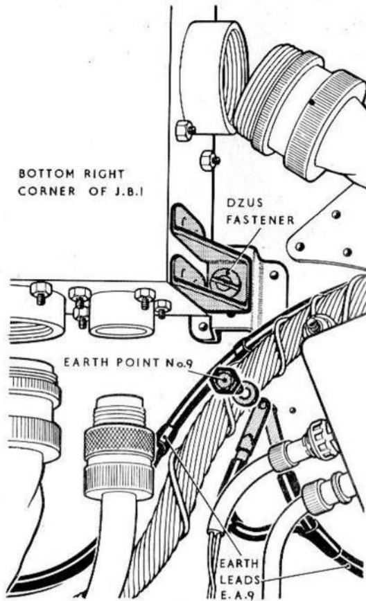
FIG.1 J.B.I LOWER ATTACHMENTS AND EARTH POINT No.9
