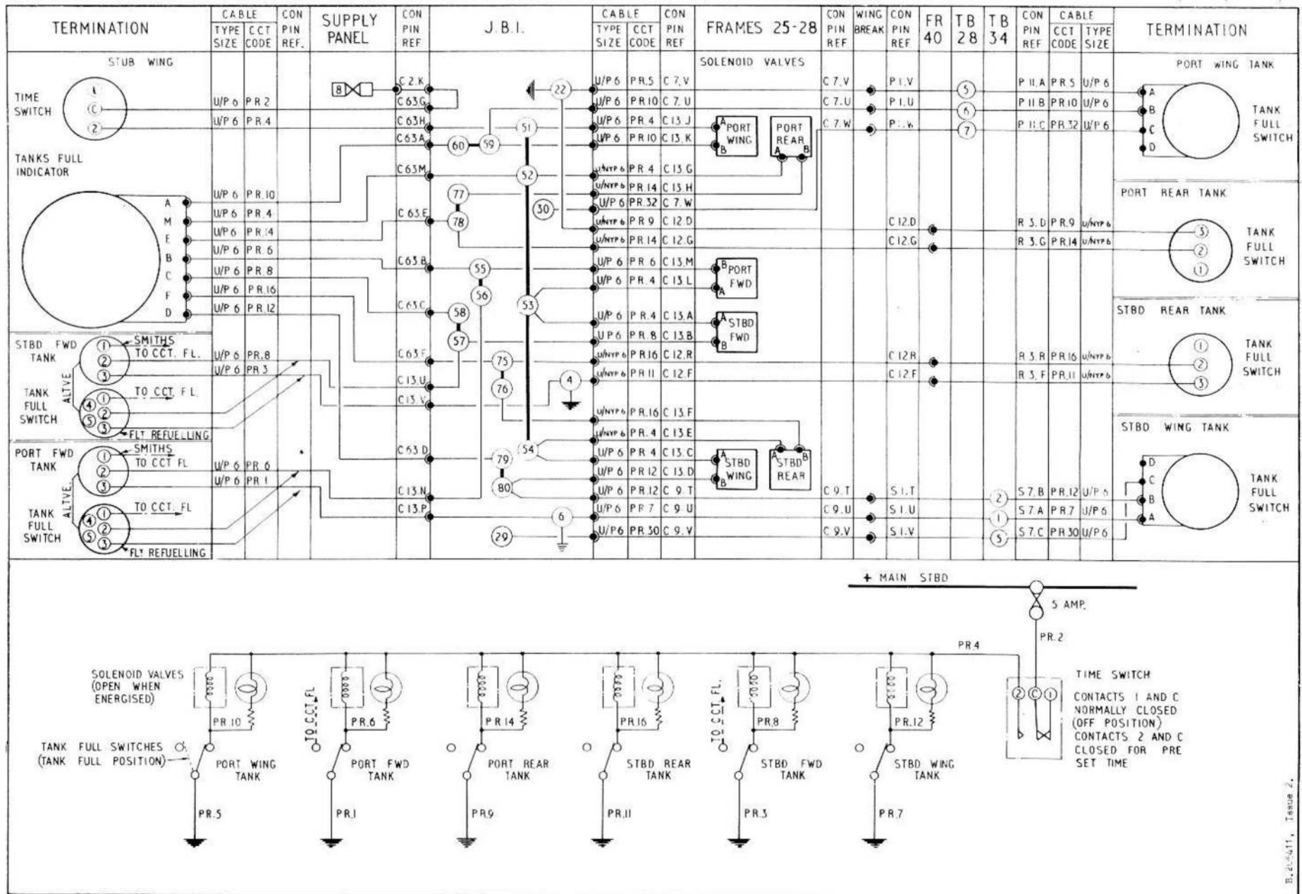
FIG. 2 PRESSURE RE-FUELLING
