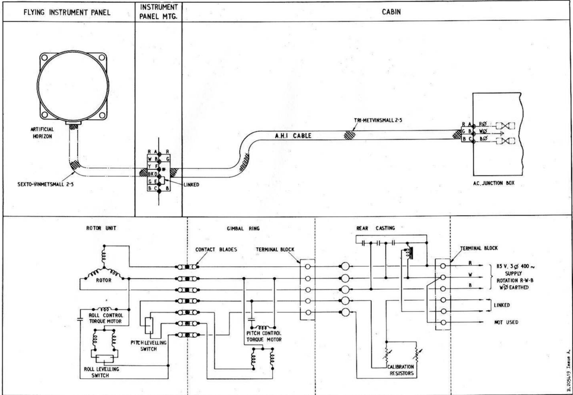
FIG. 3. ARTIFICIAL HORIZON
