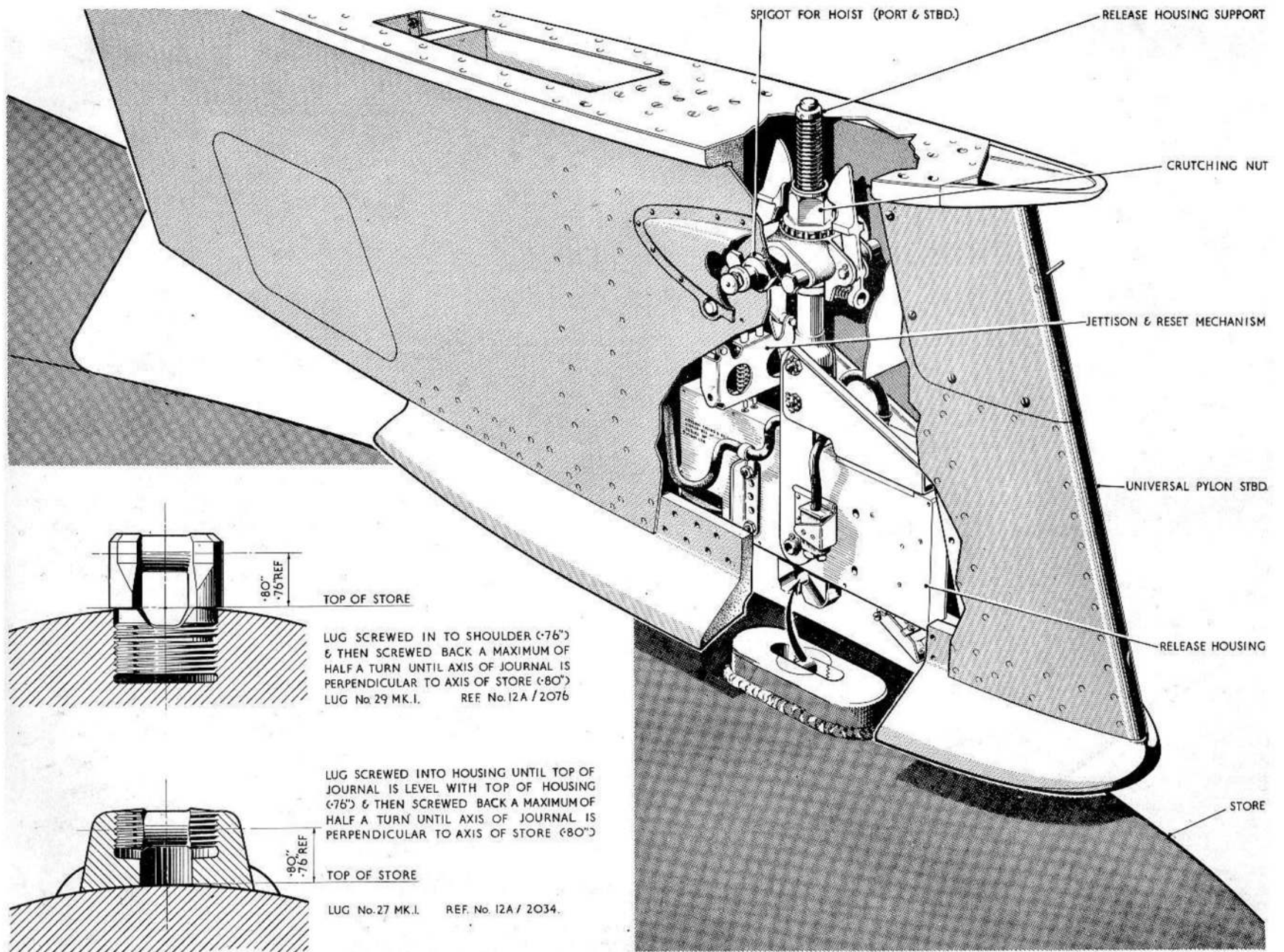
FIG. 1 BOMB INSTALLATION
