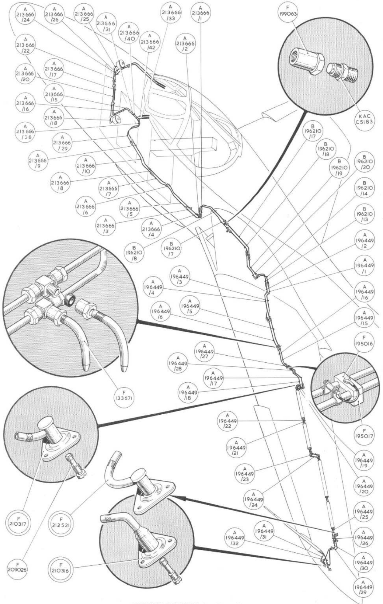
PITOT INSTALLATION
