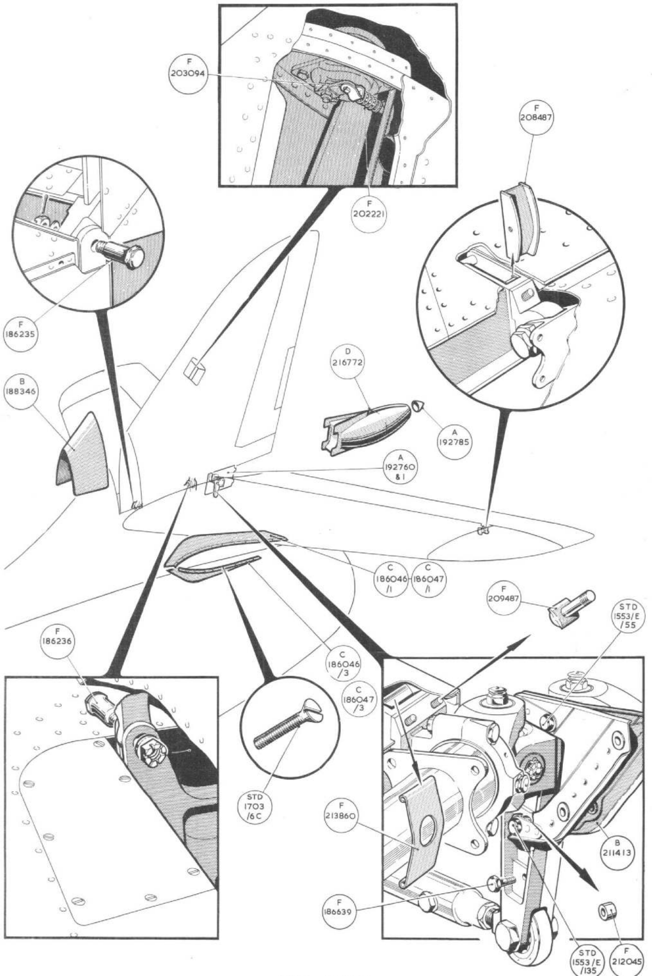
TAIL UNIT
