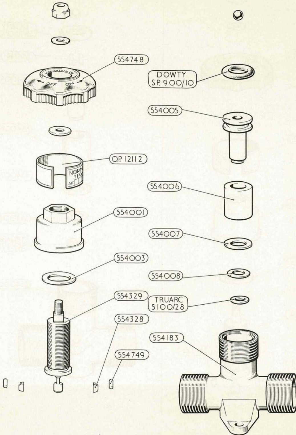
VALVE, MANUAL CONTROL
