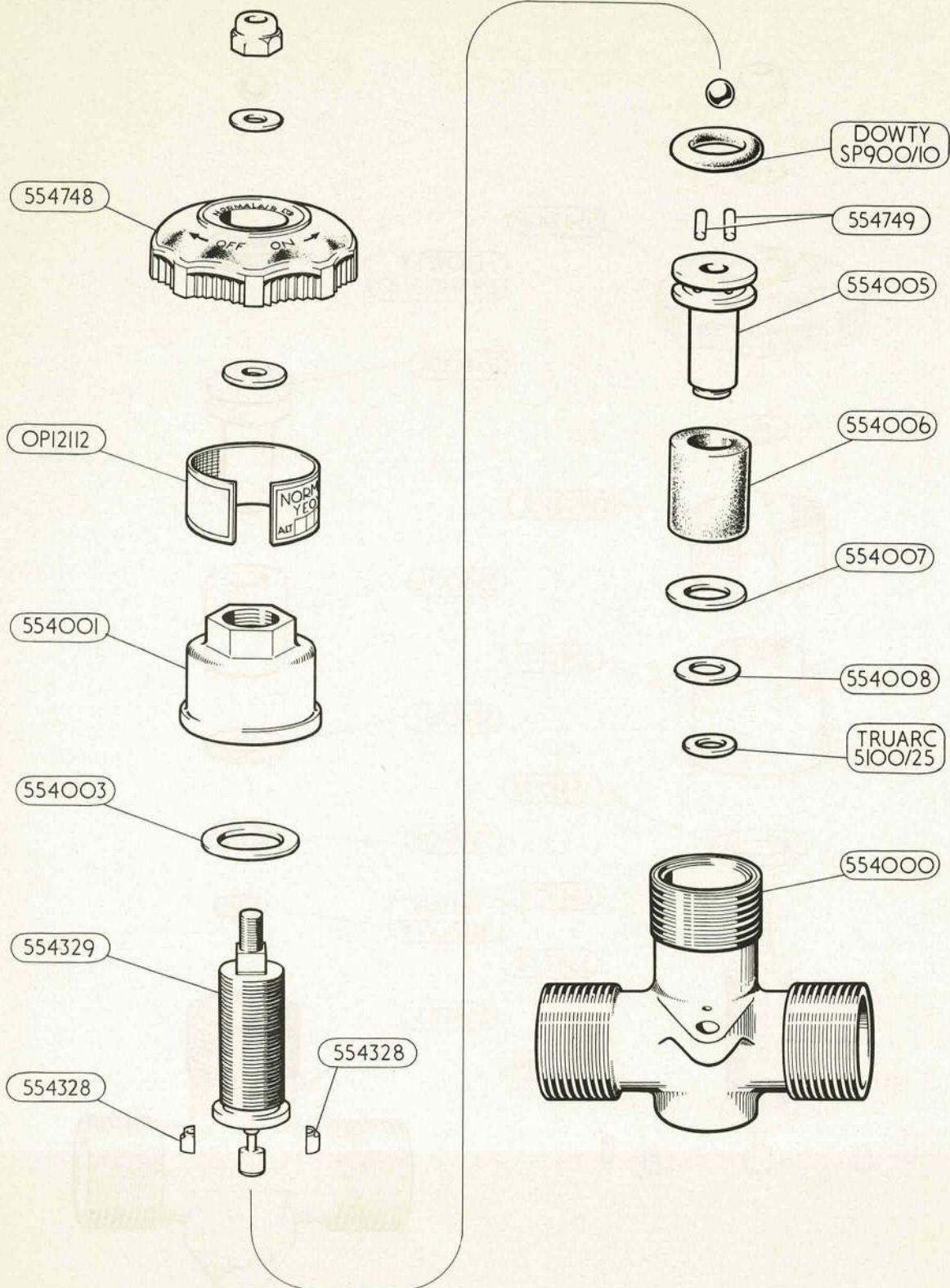
VALVE. MANUAL CONTROL.
