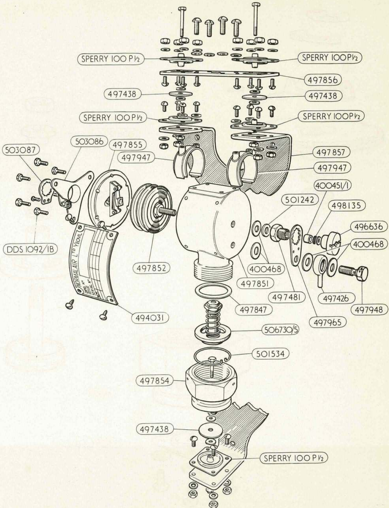
VALVE , REDUCING
