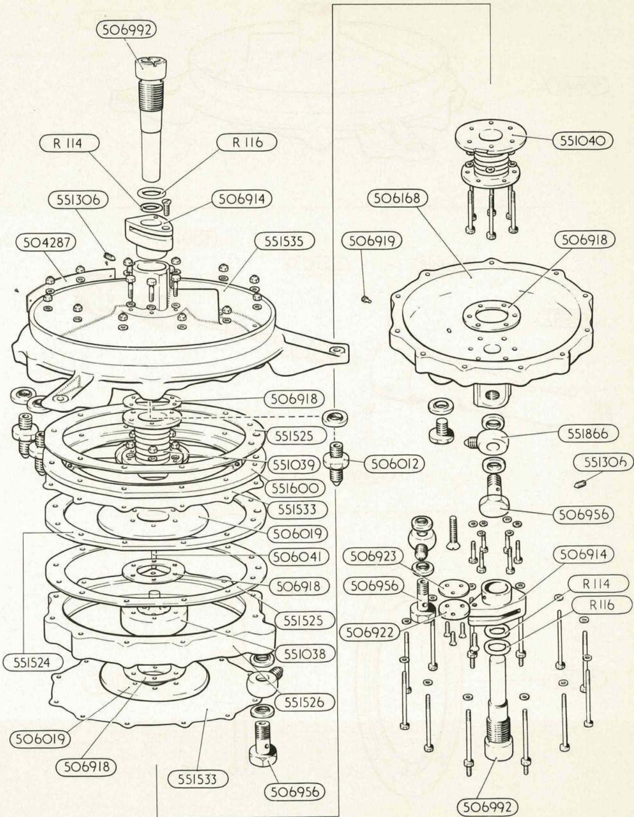
VALVE, RELAY
