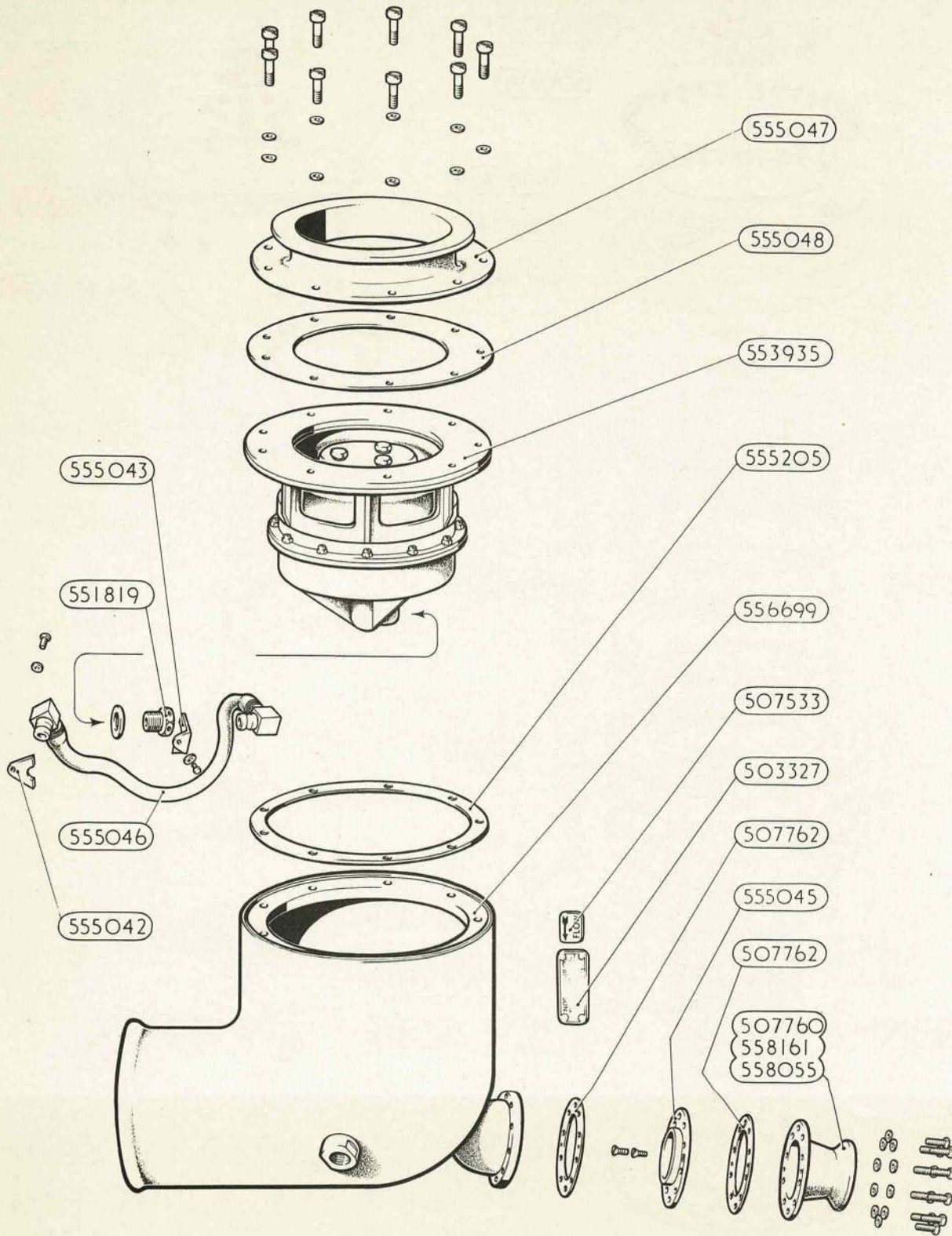
VALVE, DISCHARGE.
