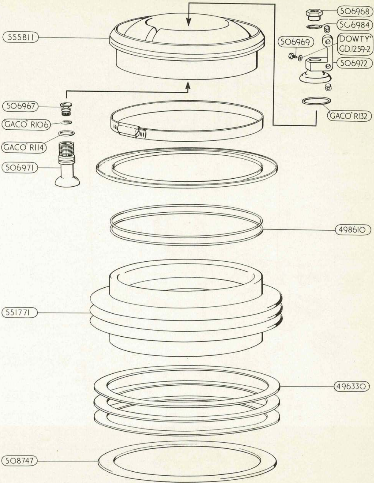
BELLOWS ASSEMBLY
