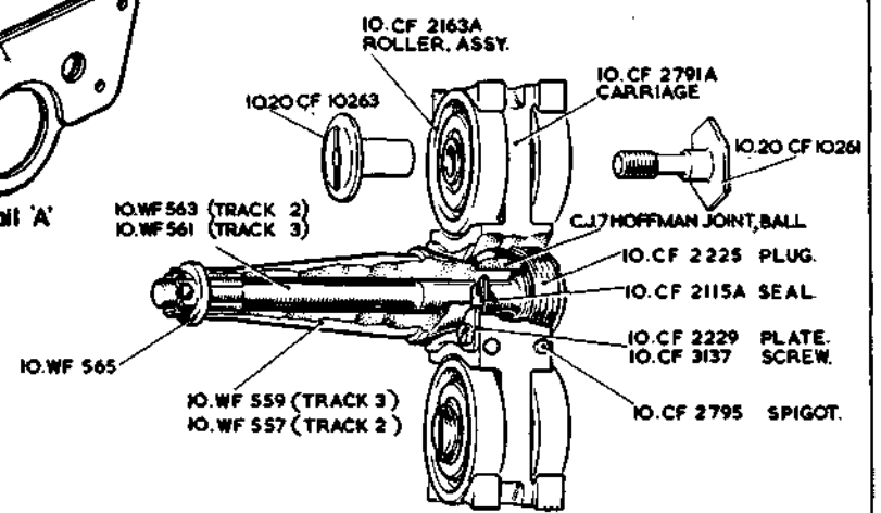
BOGIE, TORQUE TRACK, ASSEMBLY. 10.20 CF 10281A No.2 10.20 CF 10283A No.3
