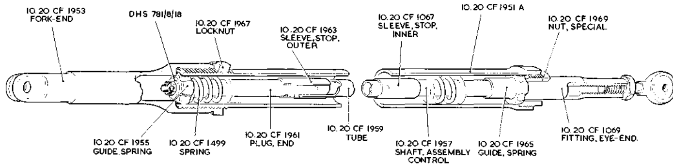
STRUT SPRING, FLAP CONTROL, ASSEMBLY. (DRG.No IO.20 CF 1949A)
