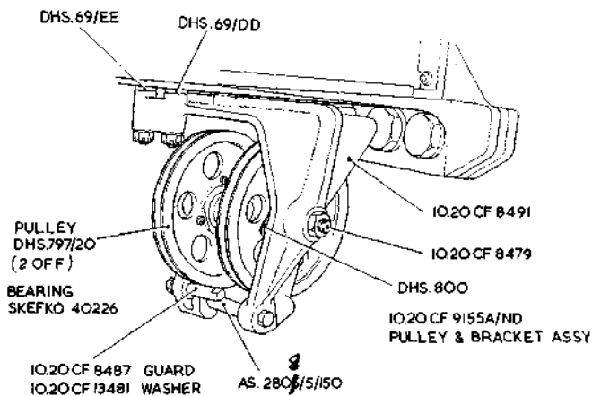
BRACKET, PULLEY AILERON CONTROL FRONT SPAR INBOARD STBD. GROUP. (DRG. No. IO.20 CF 8489)
