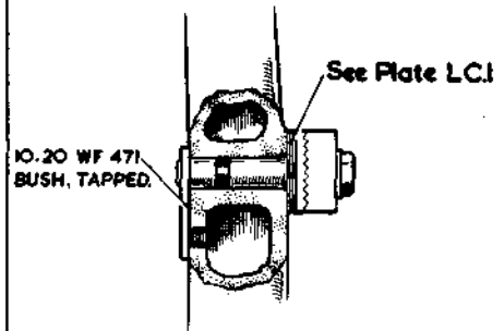
Sections of Flap Lever. 10.20 WF 4059A 10.20 WF 4060A
