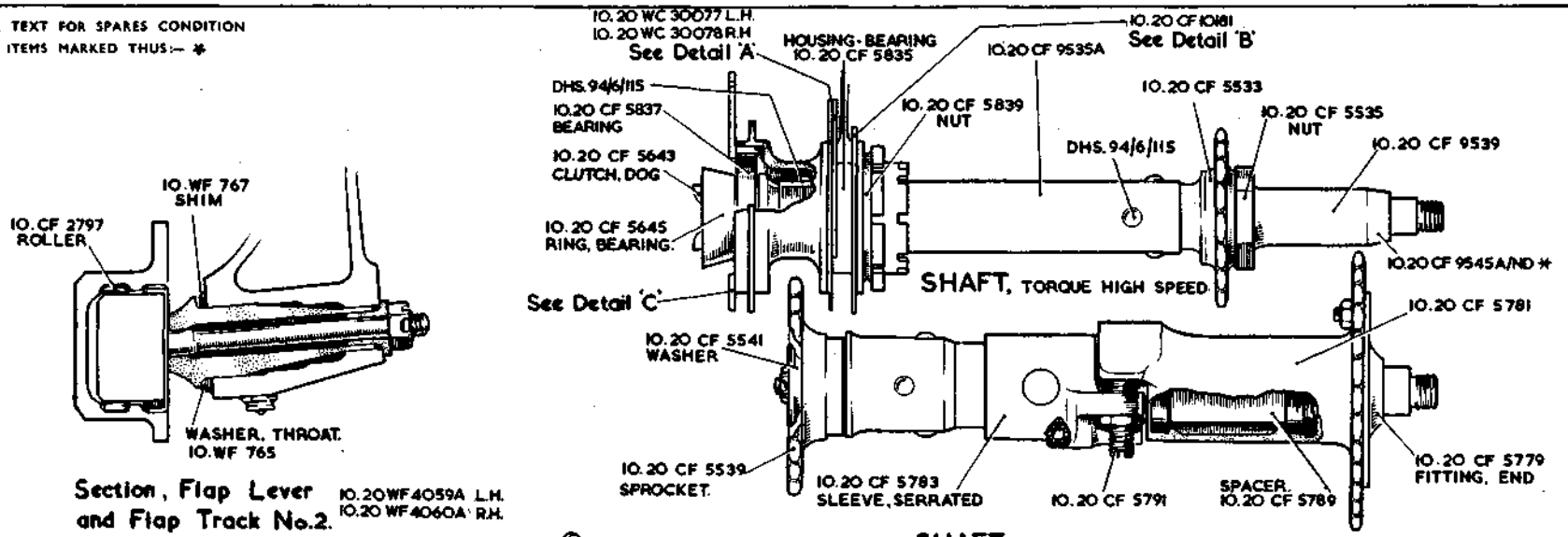
High and Low speed Shafts at Track No.3 A.
