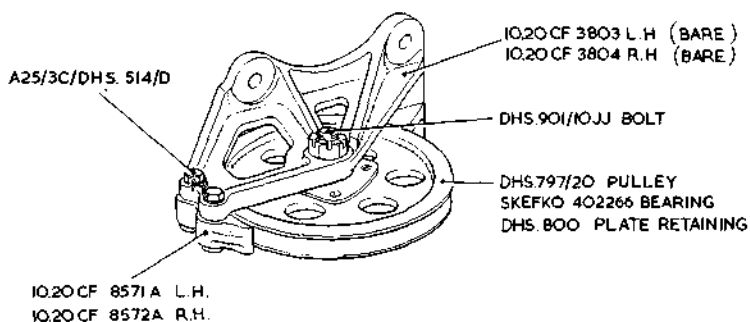
BRACKET, PULLEY, AT OUTBOARD MISSILE CASTING, AILERON CONTROLS PORT & STBD GROUP (DRG. No. IO.20 CF 3807)
