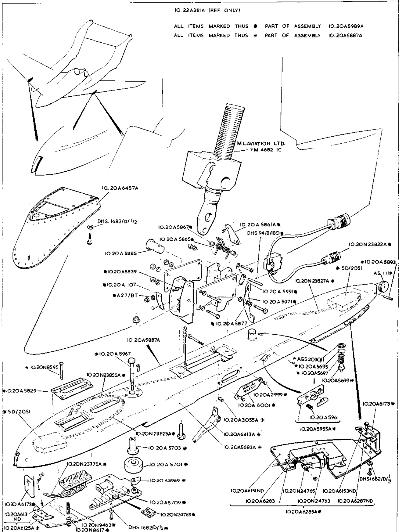
JN. 1. EQUIPMENT SPECIAL OPERATIONAL JN. 1. ADAPTATION OF LIGHT STORES PYLON FOR CARRIAGE OF 500LB BOMBS I.A.L. 74
