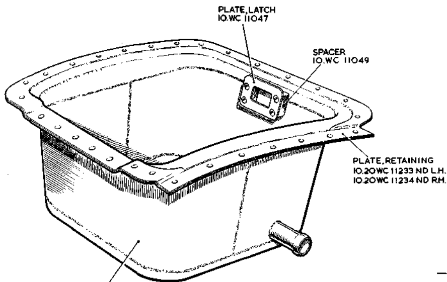
SUMP, FUEL FILLER CONNECTION TANK No.1 ASSEMBLY * 10.20WC 40873A L.H. * 10.20WC 40874A R.H.
