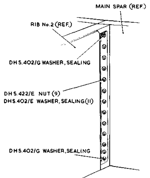
DETAIL 'C'
