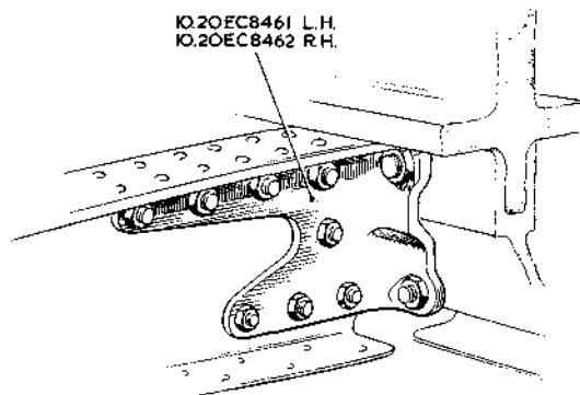
BRACKET, FRAME JOINT, BOTTOM COWLING STN. 338'10 - 339'84
