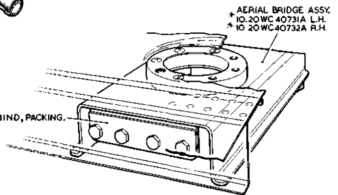
AERIAL BRIDGE, TO TOP CENTRE FAIRING. DRG No 10.20WC 40743A
