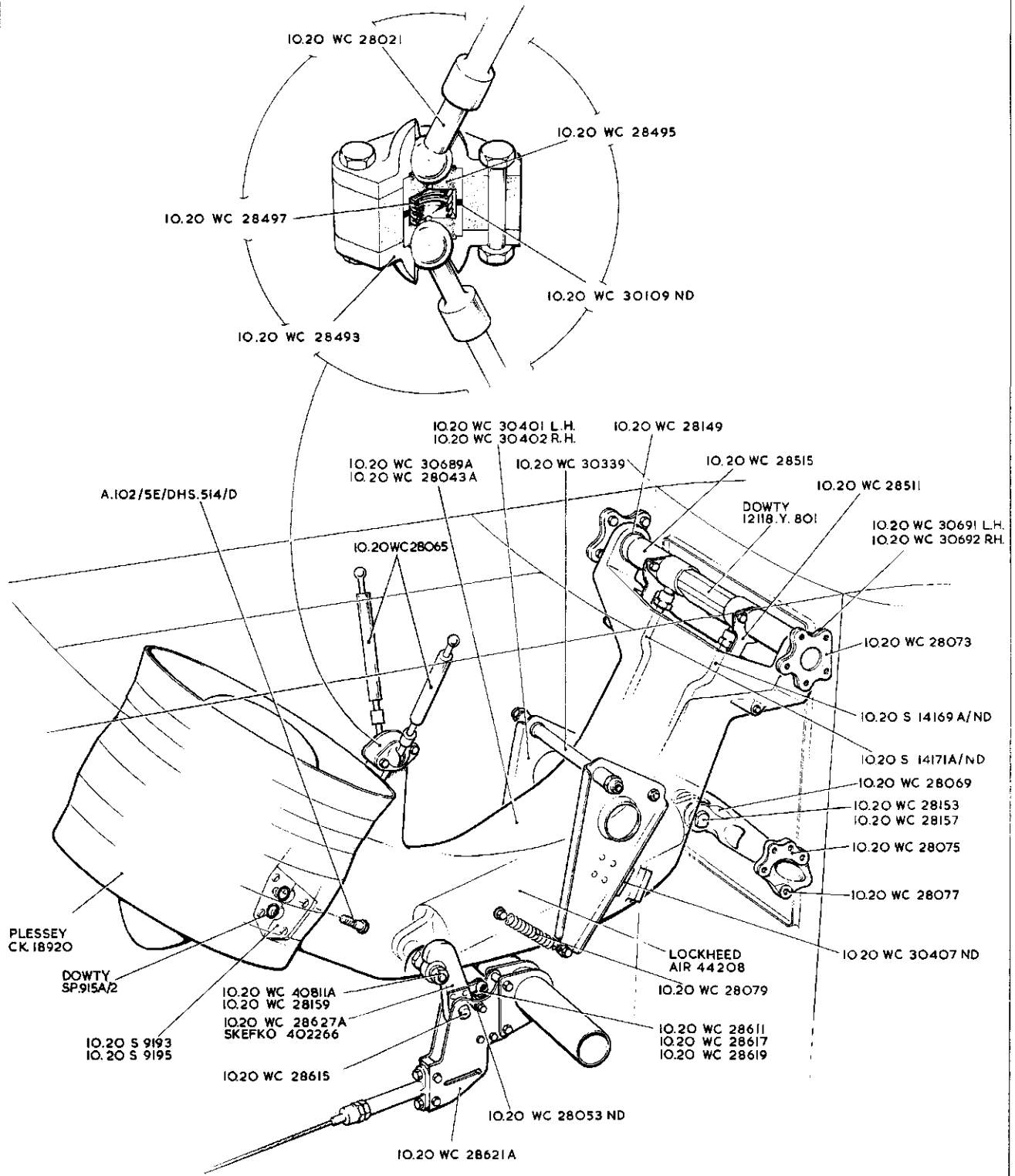
RAM AIR TURBINE. (DRG. No. IO.20 WC 28039) (MOD. 216)
