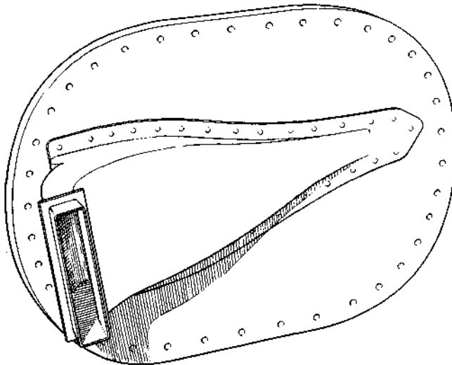
COVER, ACCESS, FLUSH AIR INTAKE, ASSY. IO.20TB 1067A PORT OUTBD, STBD. INBD. IO.20TB 1068A STBD. OUTBD.
