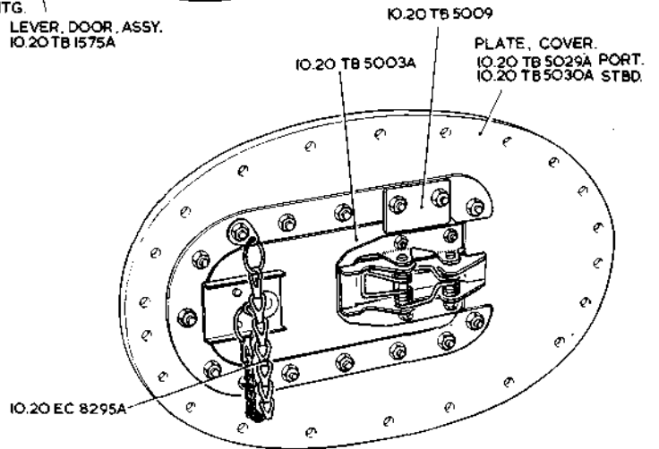
COVER-PLATE, ACCESS, FOR HANDHOLE, ASSY. IO.20TB 5031A PORT IO.20TB 5032A STBD.
