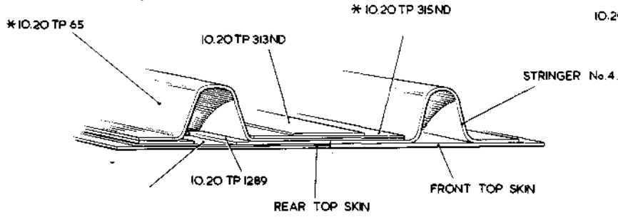
SECTION THROUGH TOP SKIN AT RIB No. 3.
