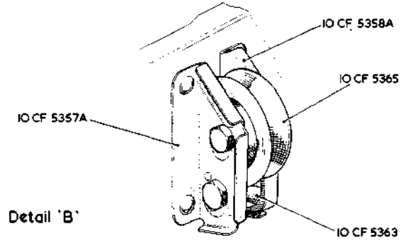
BRACKET, PULLEY & BOBBIN. RIB No. 4.
