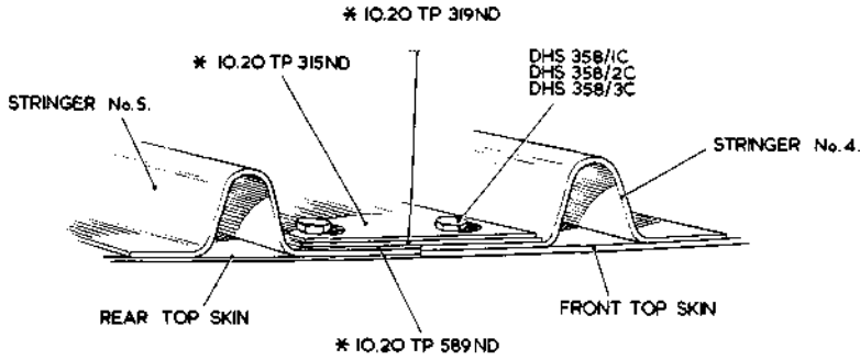
SECTION THROUGH TOP SKIN BETWEEN RIBS Nos 3 & 4
