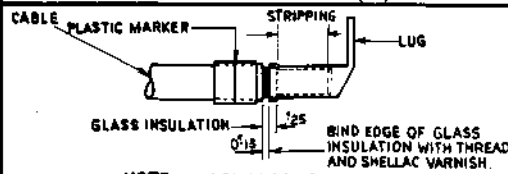
DETAIL 'N' R.C. CABLE HOLDER TERMINAL (1/4)
