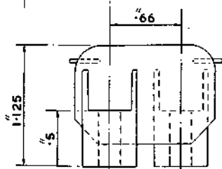
CODED EXAMPLE 20 WAY BLOCK
