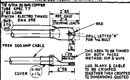
DETAIL 'R' PREN. 50 AMP HEAVY DUTY
