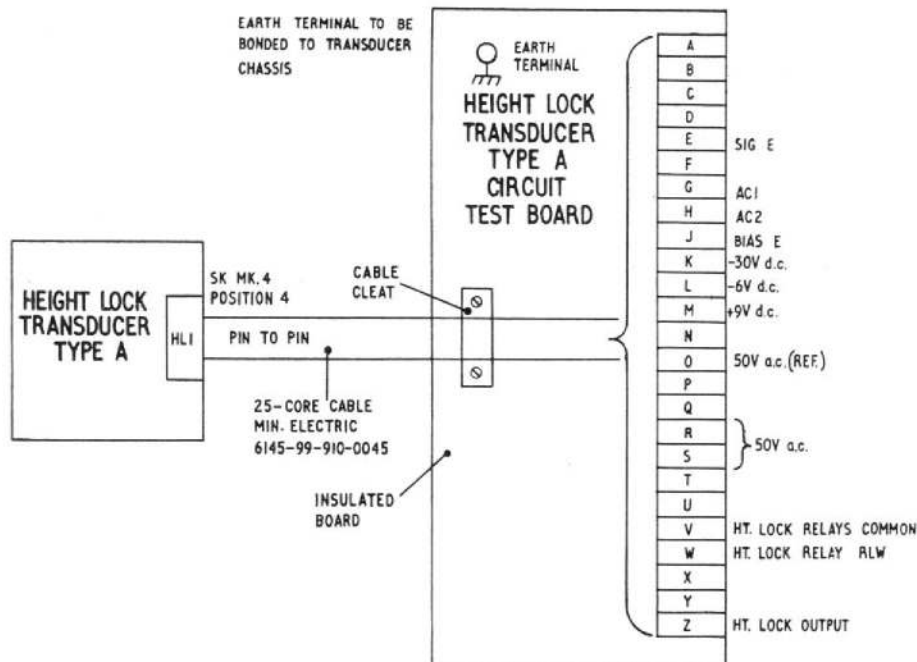
Fig. 1. Transducer connected to circuit test board
