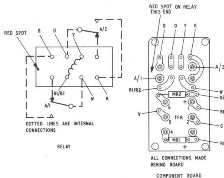
Fig. 2. Relay S2 and component board
