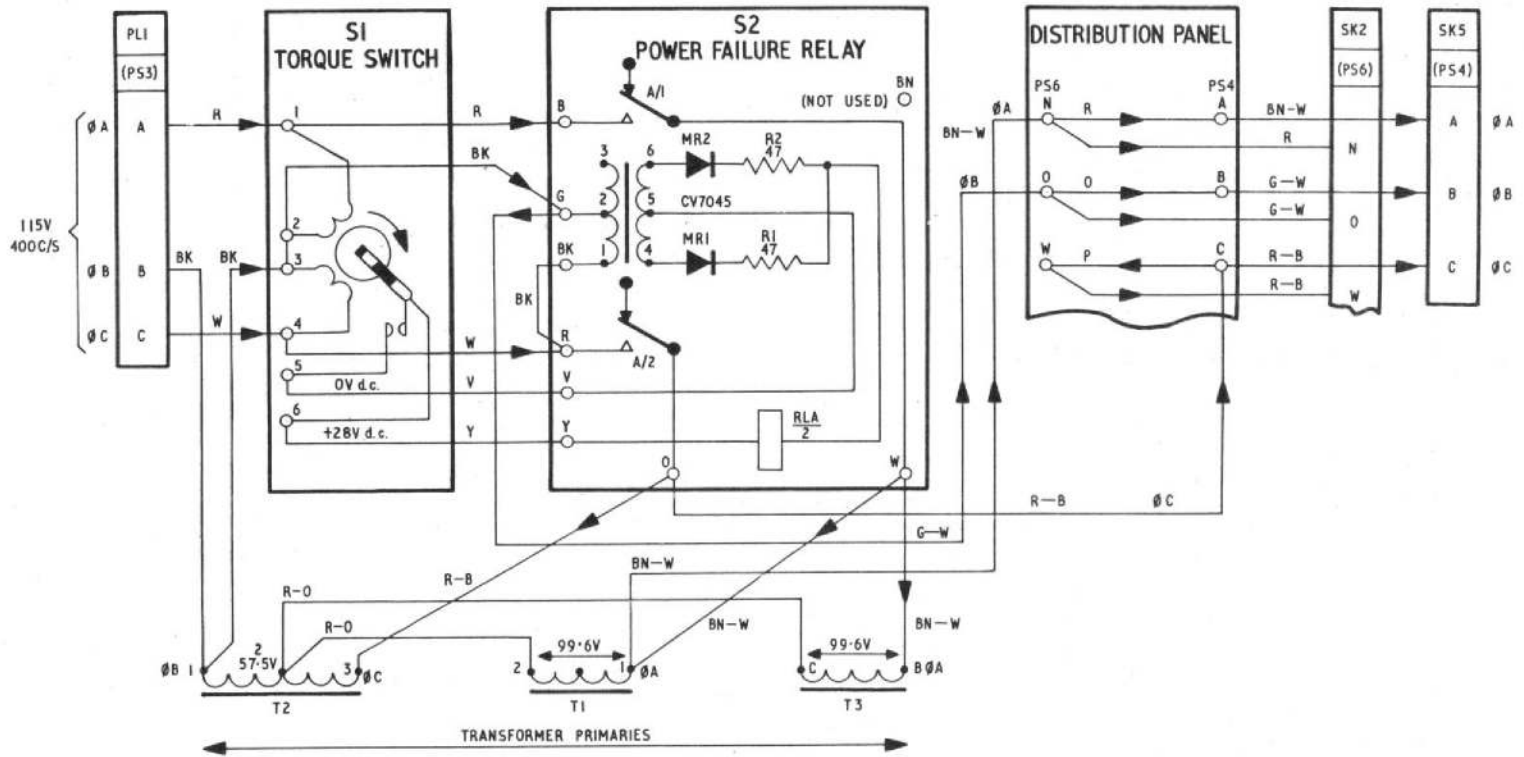
Fig. 1. 115V routing and input to transformers
