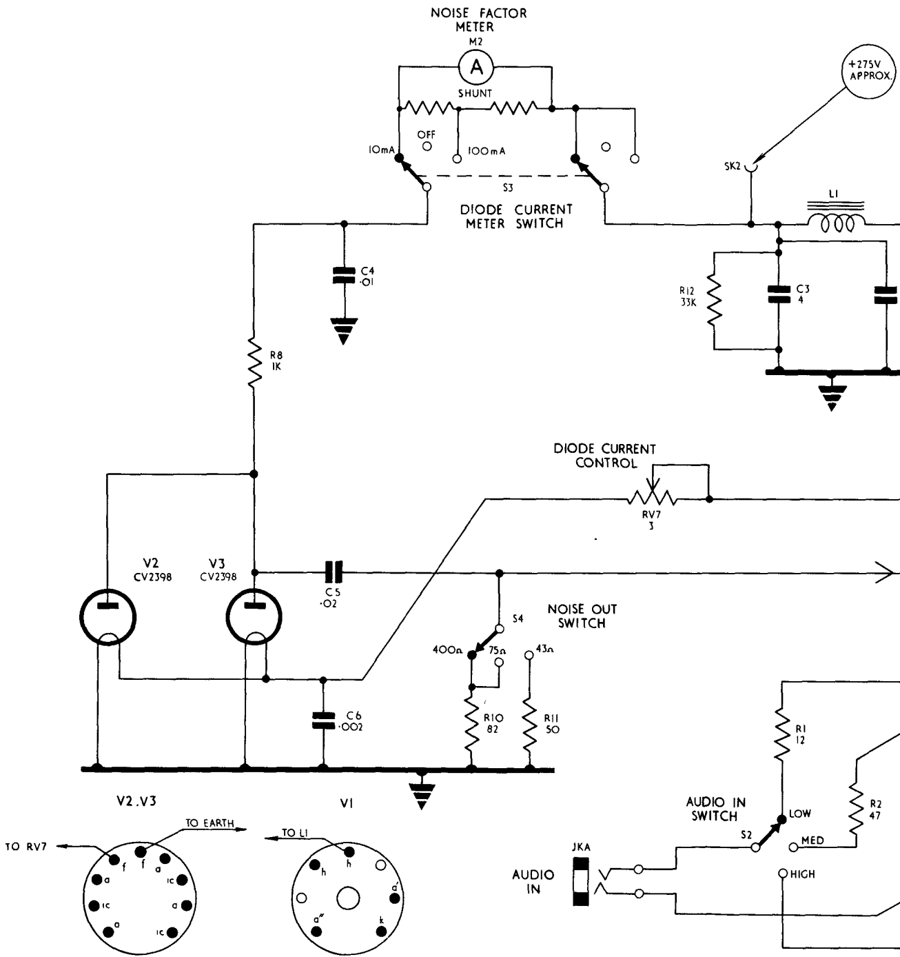
VALVE BASE CONNECTIONS
