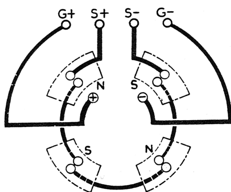
CLOCKWISE ROTATION
