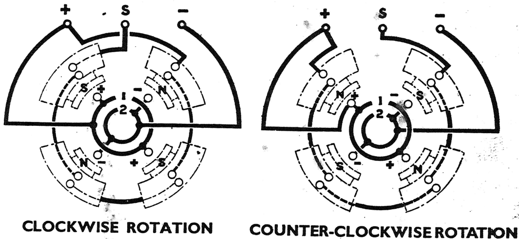
Fig. 3.—Diagram of field connections, K and KX generators, looking at commutator end
