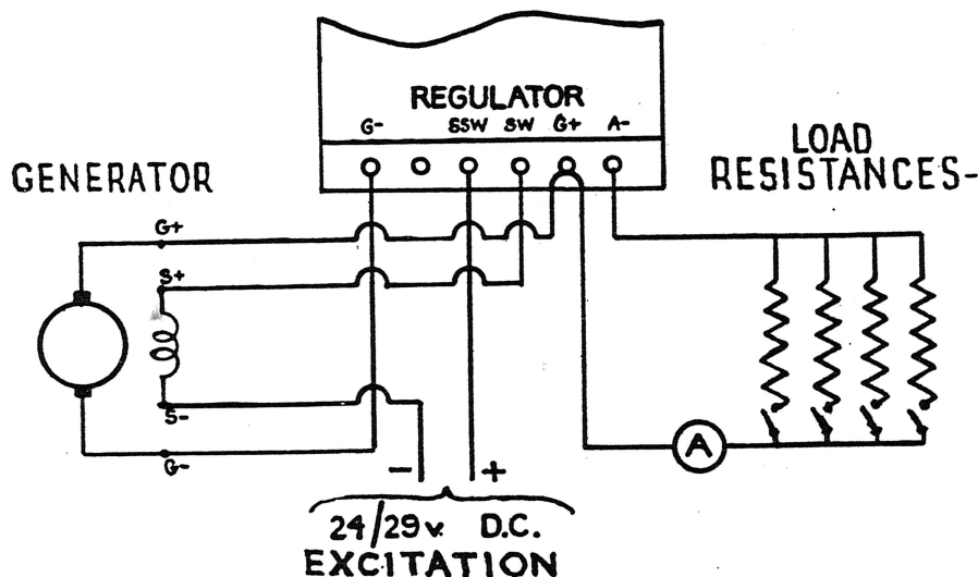
Fig. 10.—Test circuit diagram, generators, types KZ1 and KZ2
