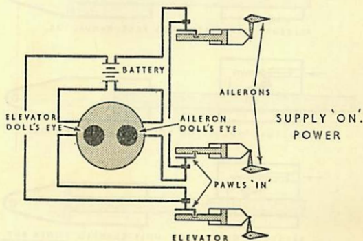
Fig. 17. Indicators—Electrical Circuits
