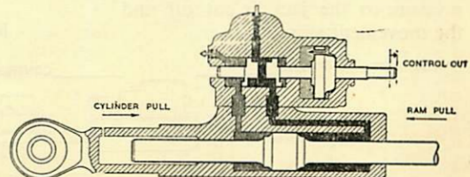
Fig. 3. Valve Action—Control Rod Out
