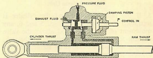
Fig. 1. Valve Action—Control Rod In
