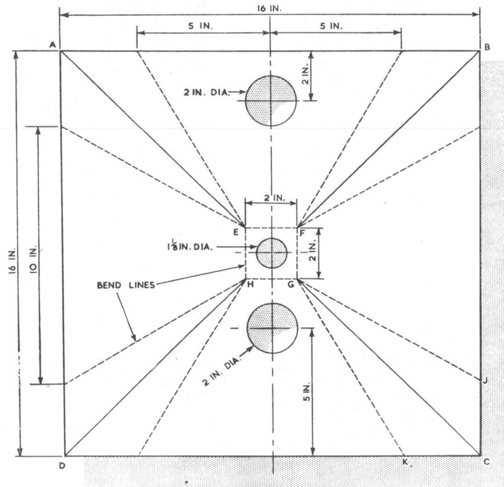
Fig. 1. Marking-out details
