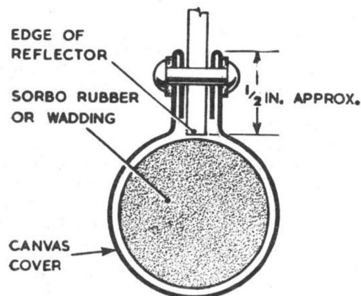
Fig. 5. Typical seal
