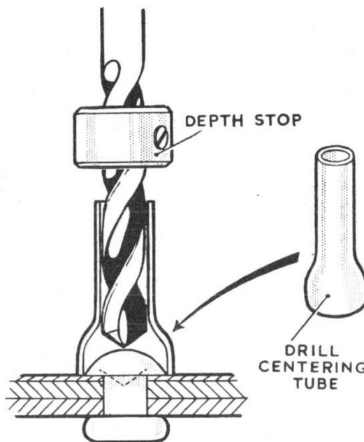
Fig. 1. Rivet removal
