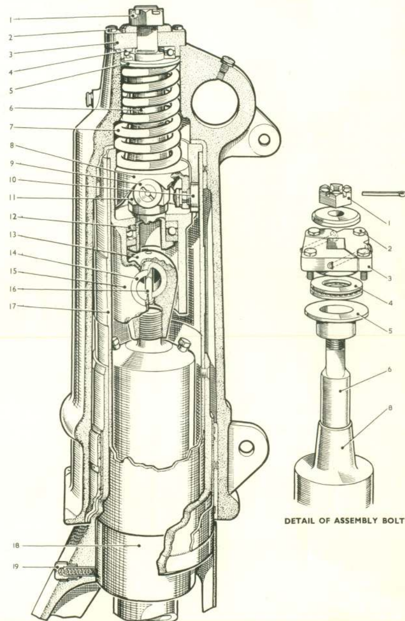
Fig. 10 Self-centring mechanism
