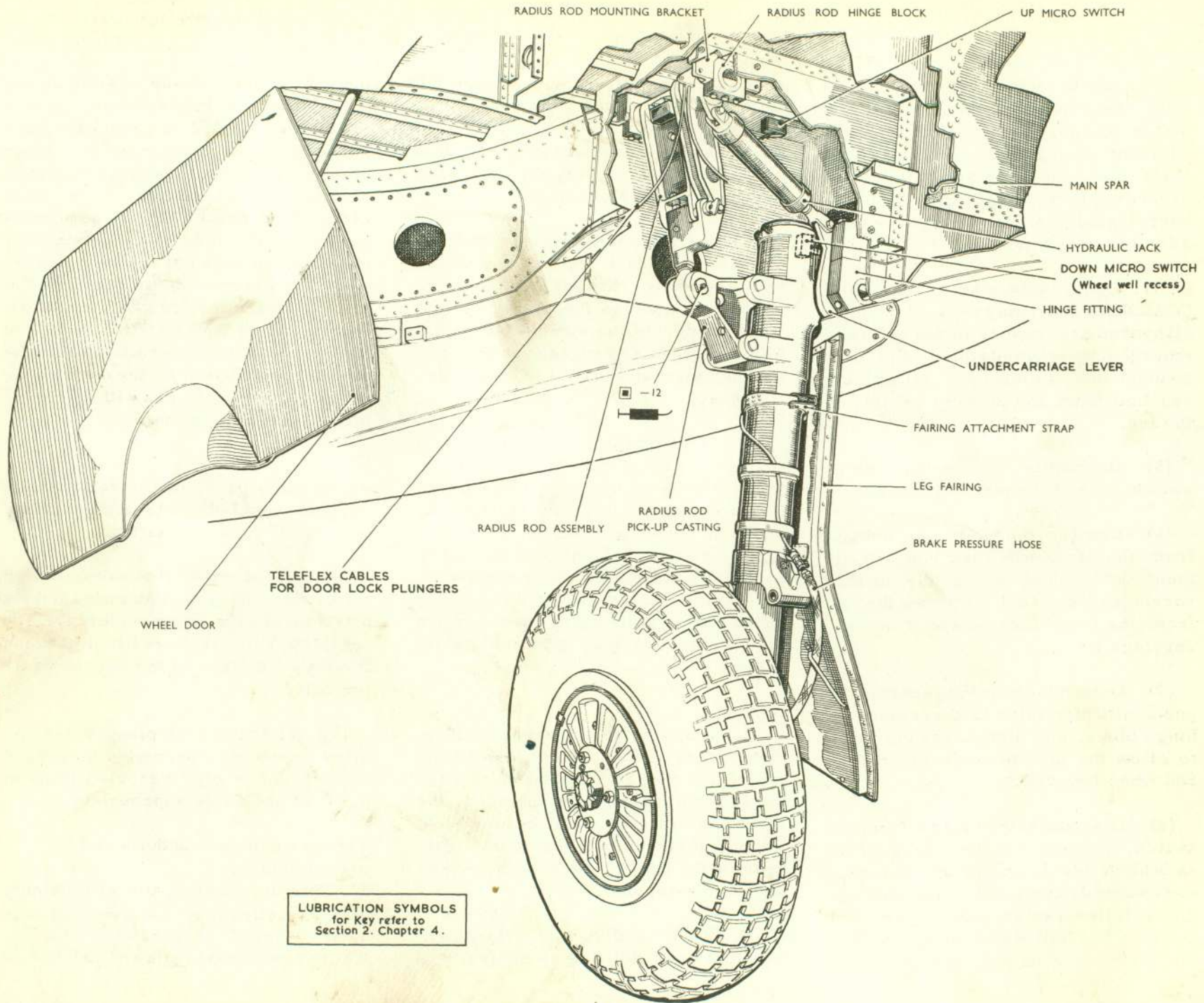
Fig. 8 Main undercarriage
