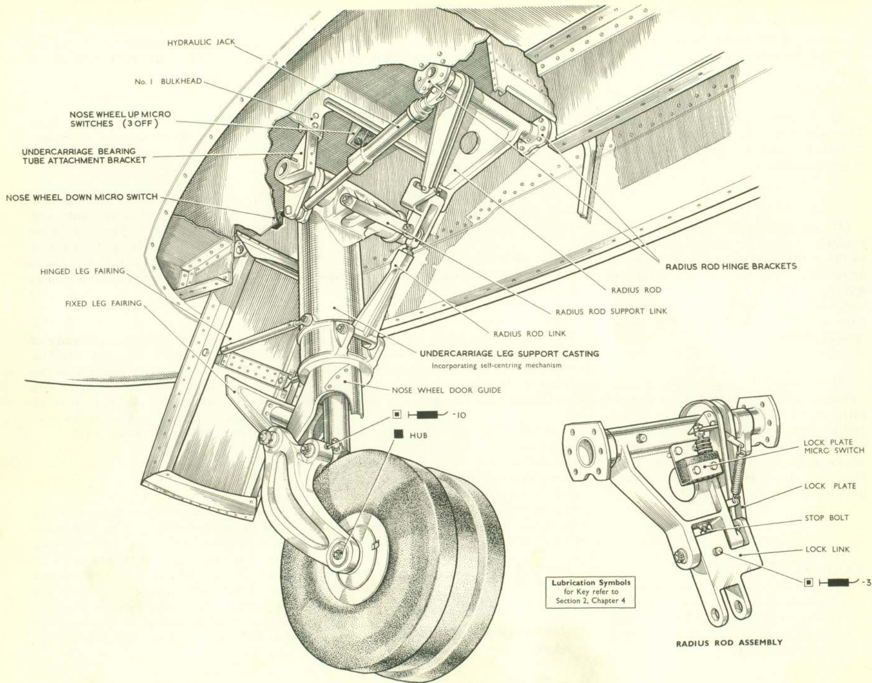
Fig. 9 Nose undercarriage
