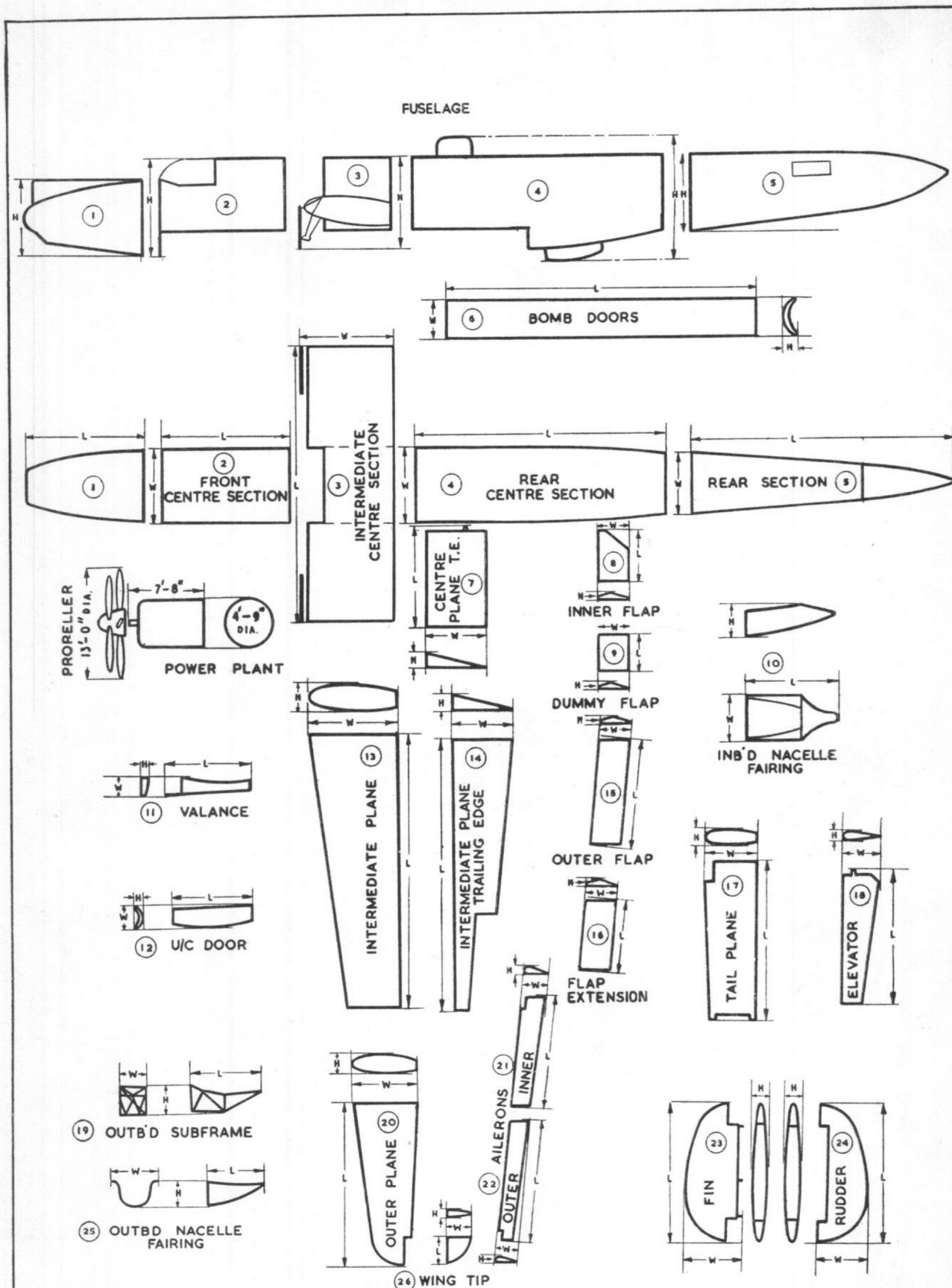
SHACKLETON G.R. MK2.- PACKING DIMENSIONS
