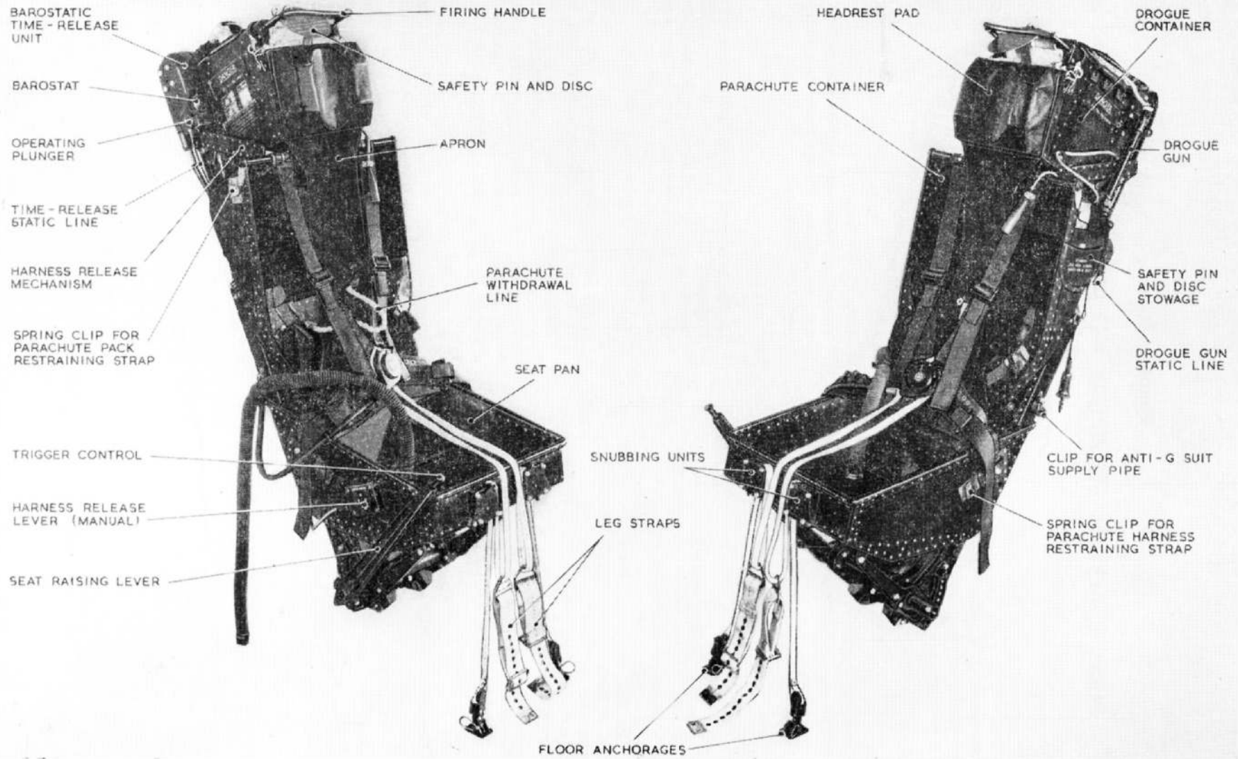
Fig. 1. Mk. 3A ejection seat (structure)
