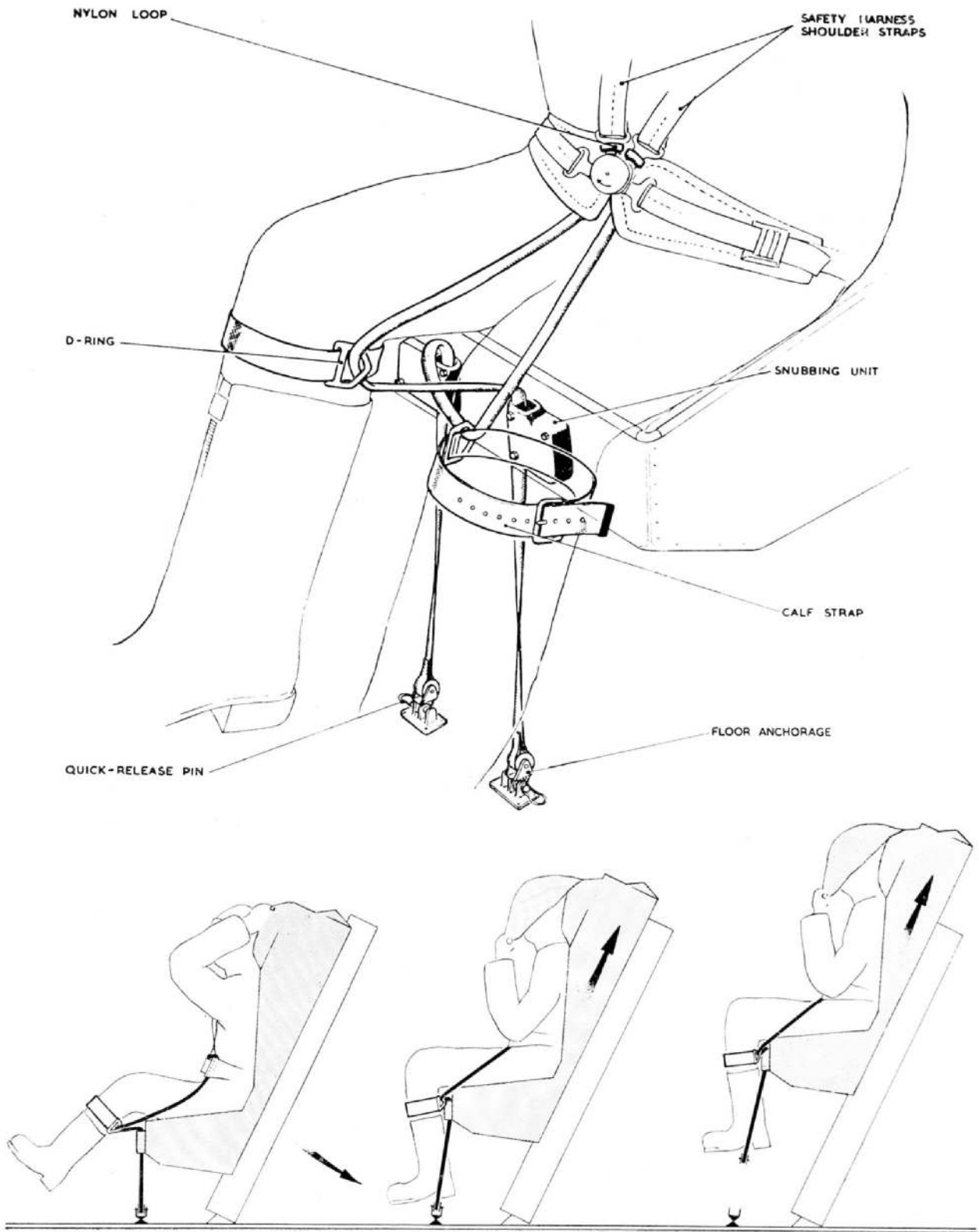
Fig. 3. Leg restraining device
