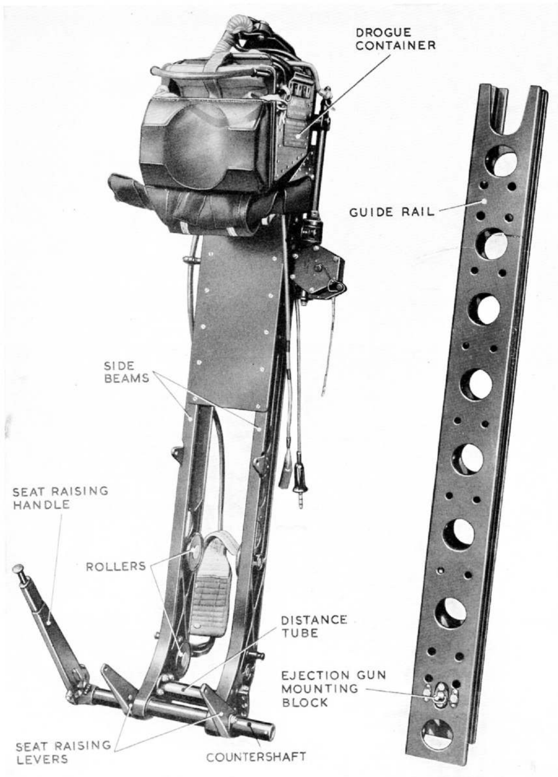
Fig. 1. Seat structure and guide rail
