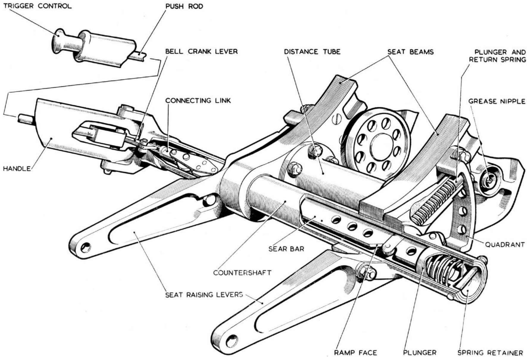
Fig. 5. Seat raising mechanism
