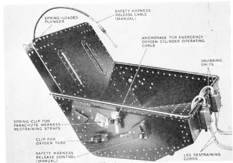
Fig. 2. Seat pan
