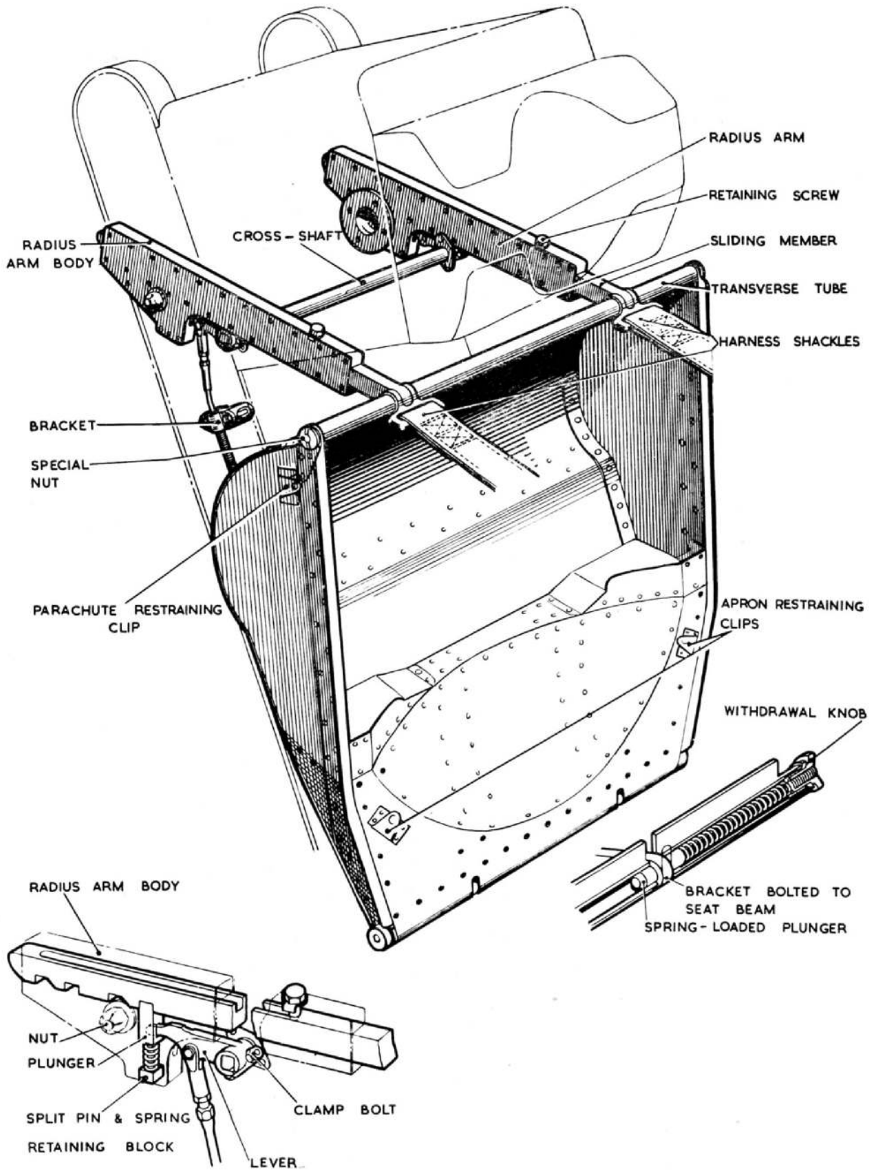
Fig. 6. Parachute container
