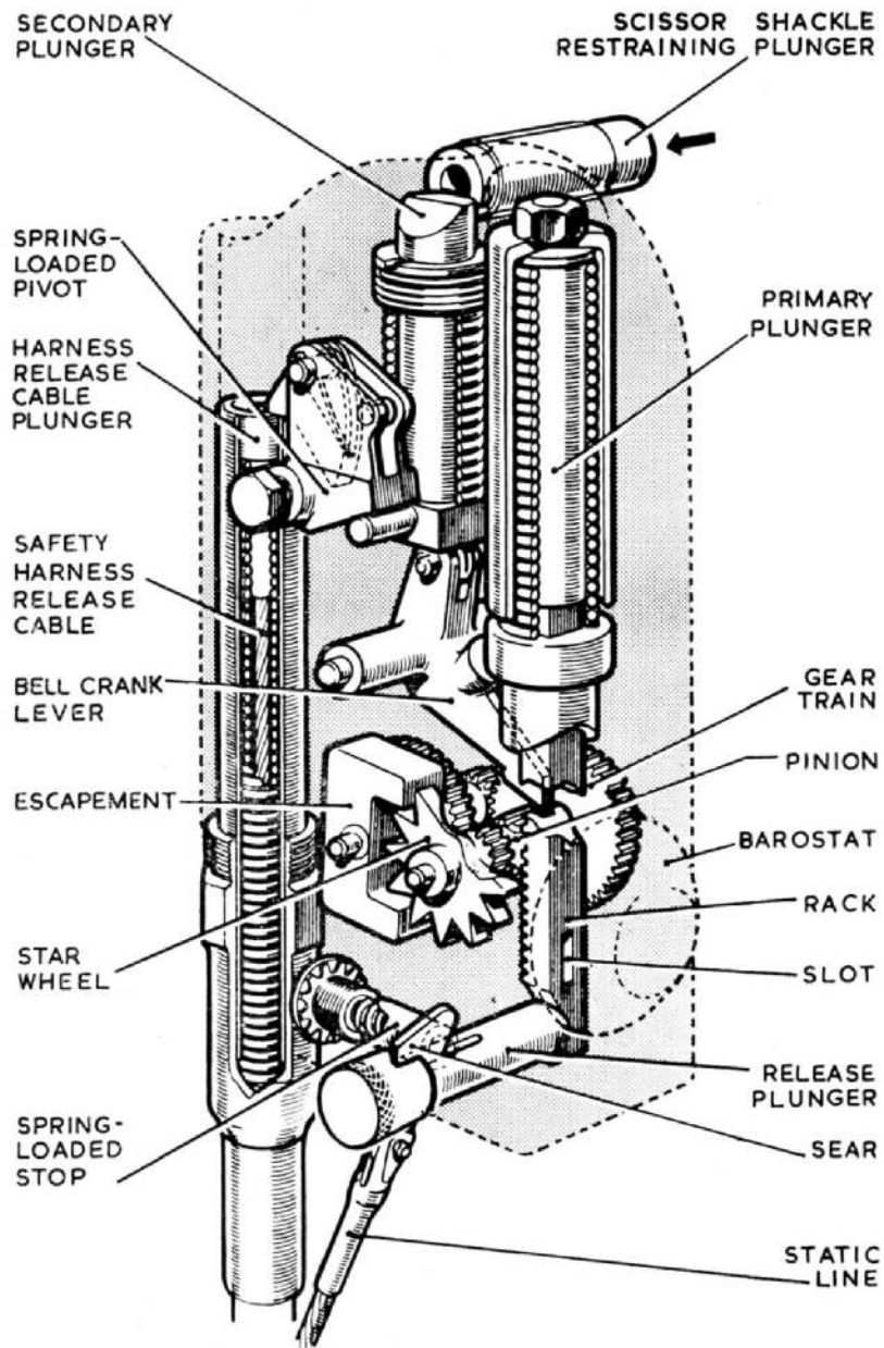
Fig. 9. Details of time-release unit
