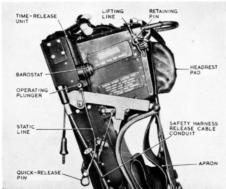
Fig. 9. Barostatic time-release unit
