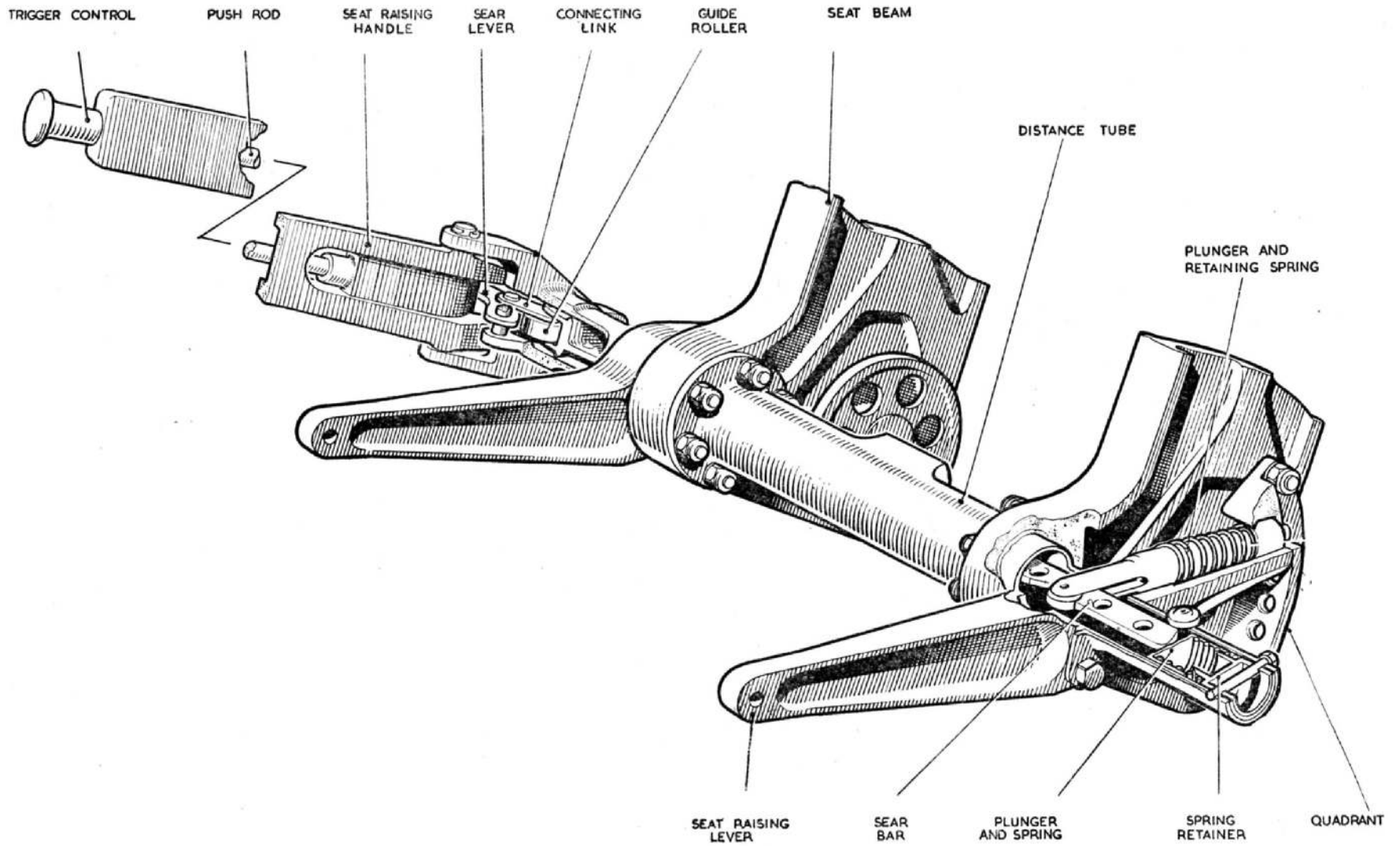
Fig. 6. Seat raising mechanism
