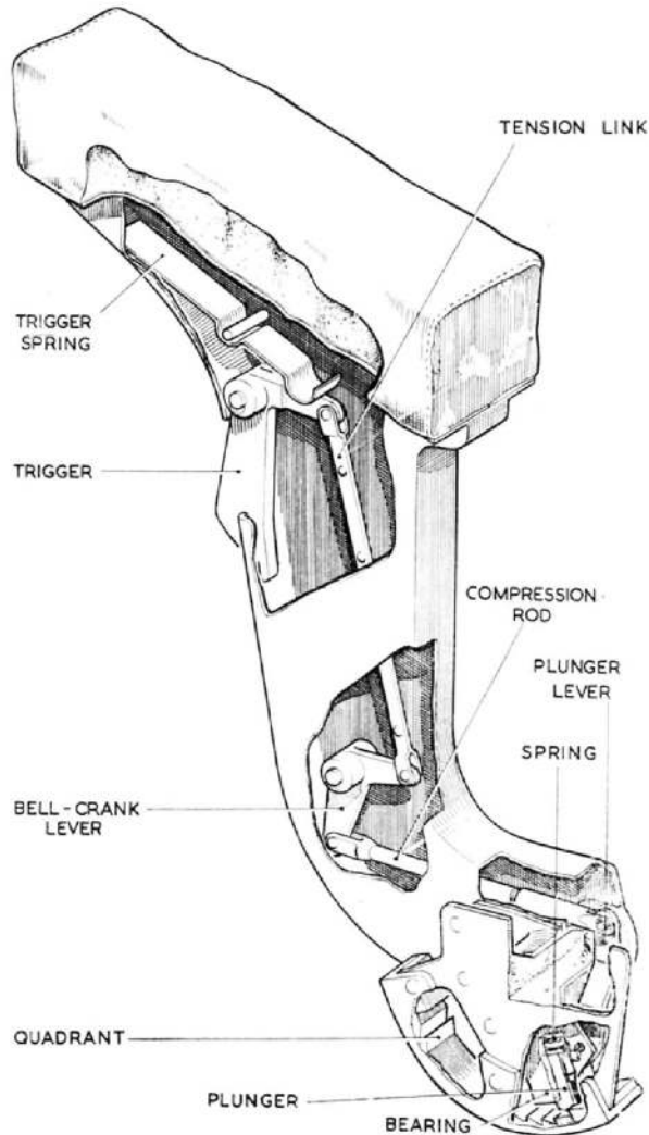
Fig. 4. Details of armrest
