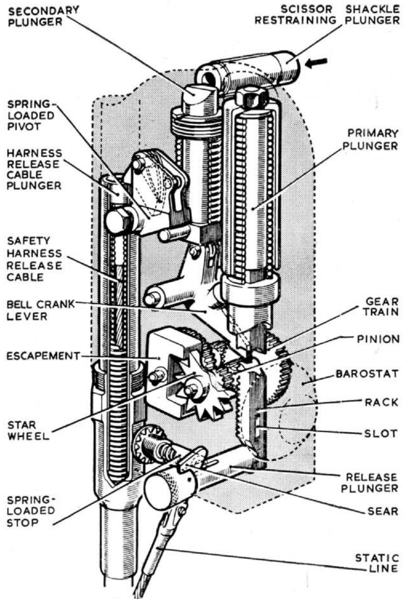
Fig. 10. Details of time-release unit
