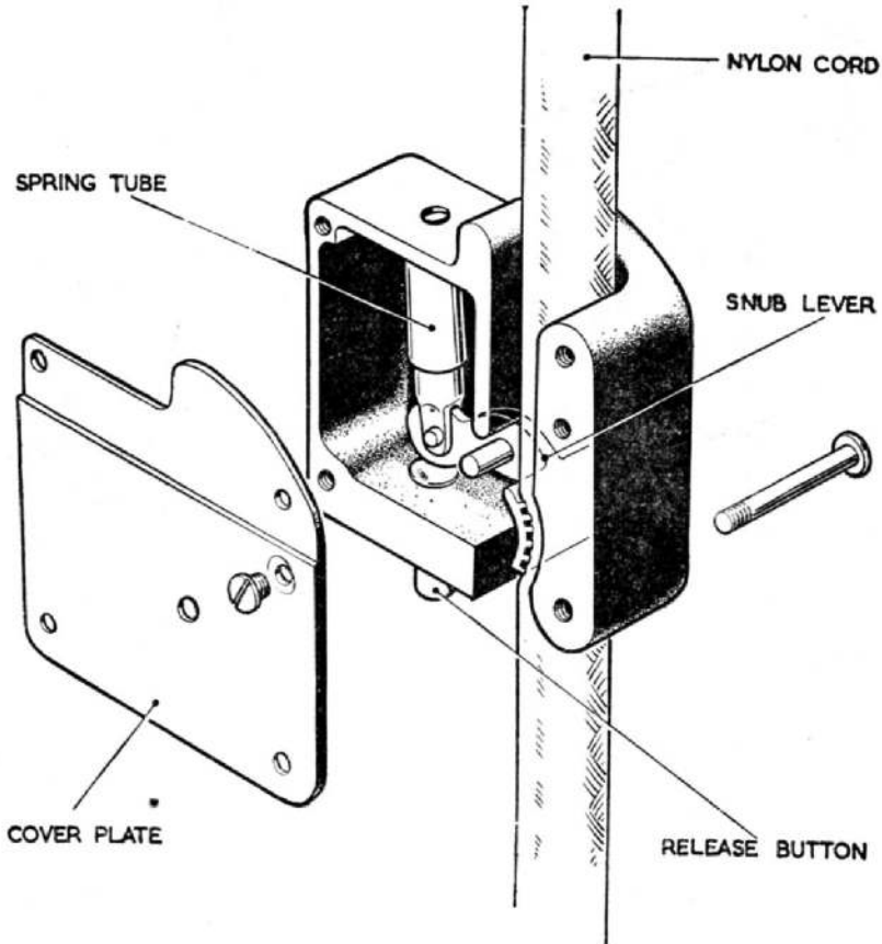
Fig. 5. Details of snubbing unit
