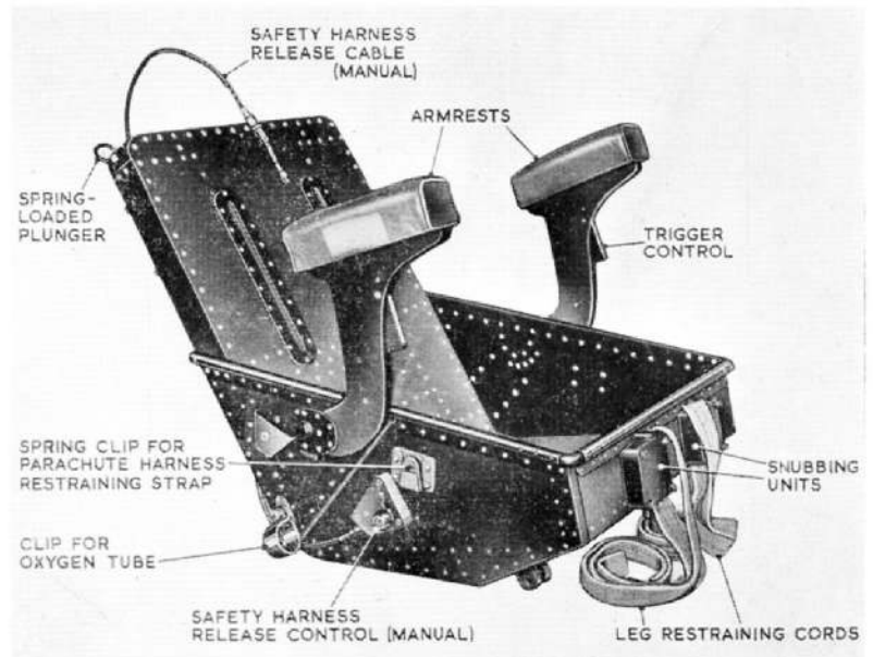
Fig. 2. Seat pan
