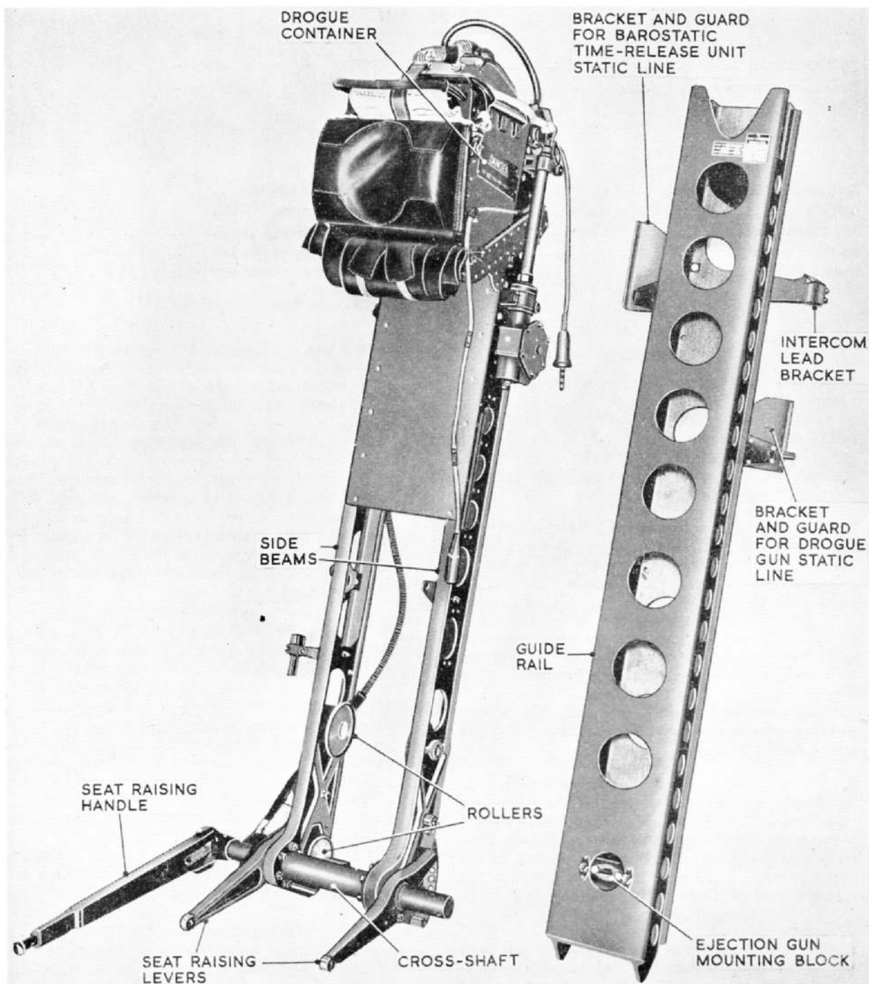
Fig. 1. Seat structure and guide rail
